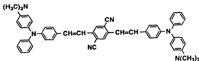
Structural formula (15)-5:
