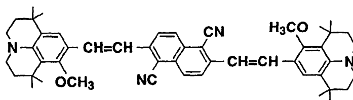
Structural formula (17)-5:
