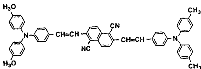
Structural formula (17)-4:
