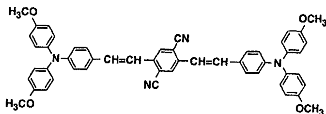
Structural formula (15)-3:
