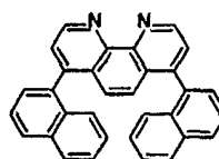
Structural formula 8:
