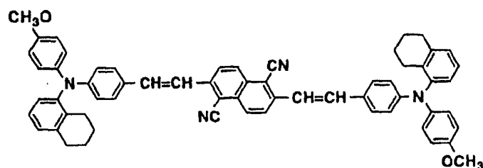
Structural formula (17)-3:
