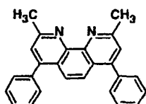
Structural formula 2:
