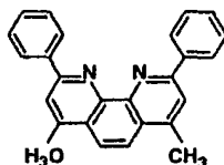
Structural formula 3:
