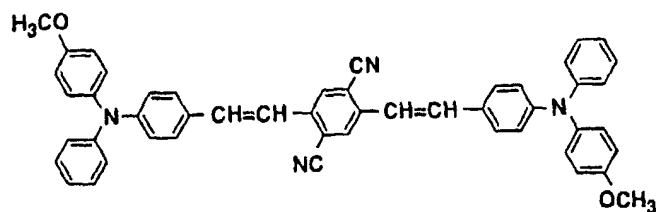
Structural formula (15)-1:
