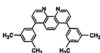
Structural formula 5:
