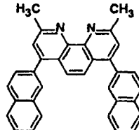
Structural formula 10:
