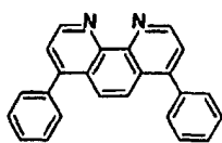
Structural formula 1:
