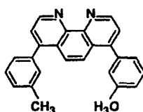
Structural formula 4:
