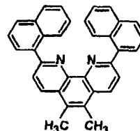
Structural formula 9:
