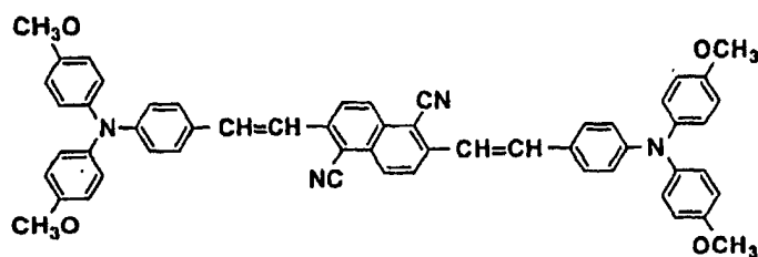
Structural formula (17)-2:
