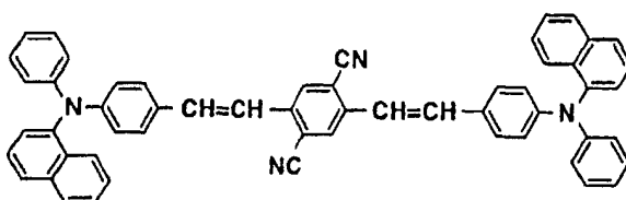
Structural formula (15)-11:
