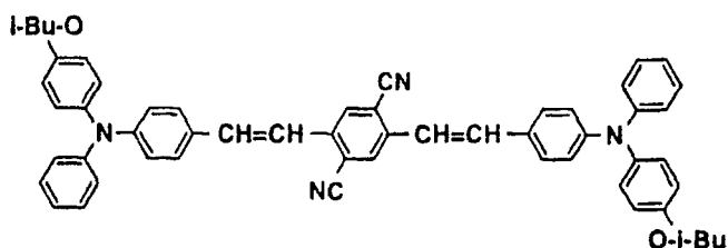
Structural formula (15)-7:
