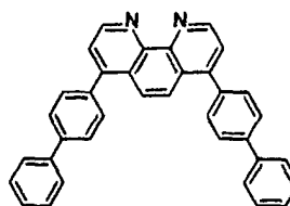
Structural formula 6:
