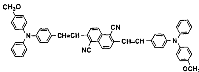
Structural formula (17)-1:
