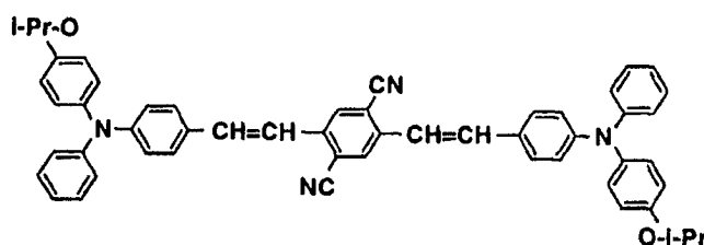
Structural formula (15)-8:
