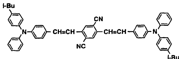
Structural formula (15)-6:
