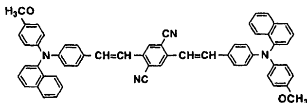
Structural formula (15)-12:
