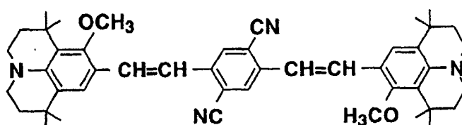
Structural formula (15)-9:
