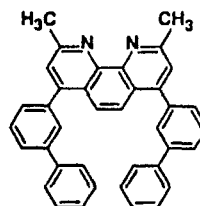
Structural formula 7:
