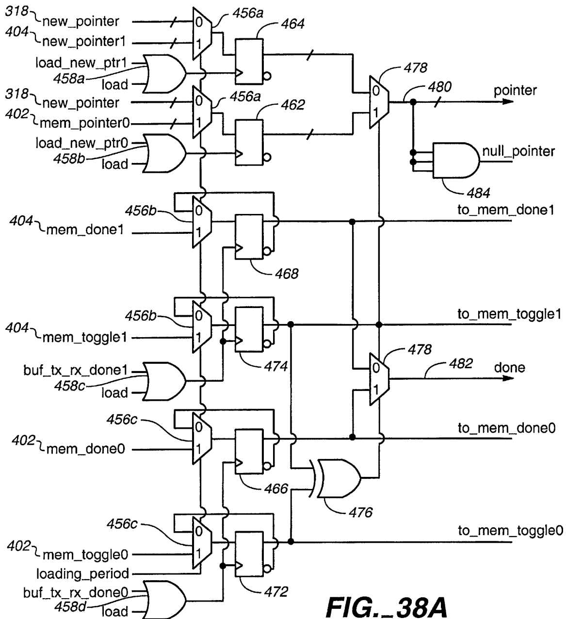
Dua Pointer Buffer Scheme 1: Hardware implementation
