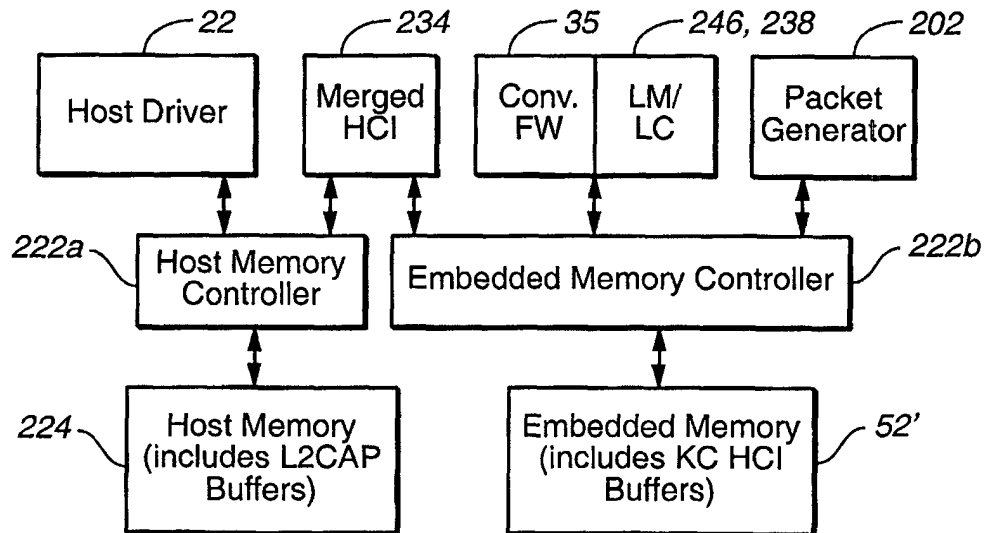
Type A-2: Host / KC Technology Bluetooth BaseBand Controller
