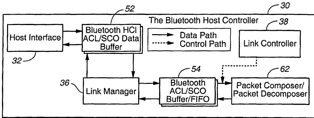
Data Flow and Buffer Scheme in the Bluetooth Host Controller
