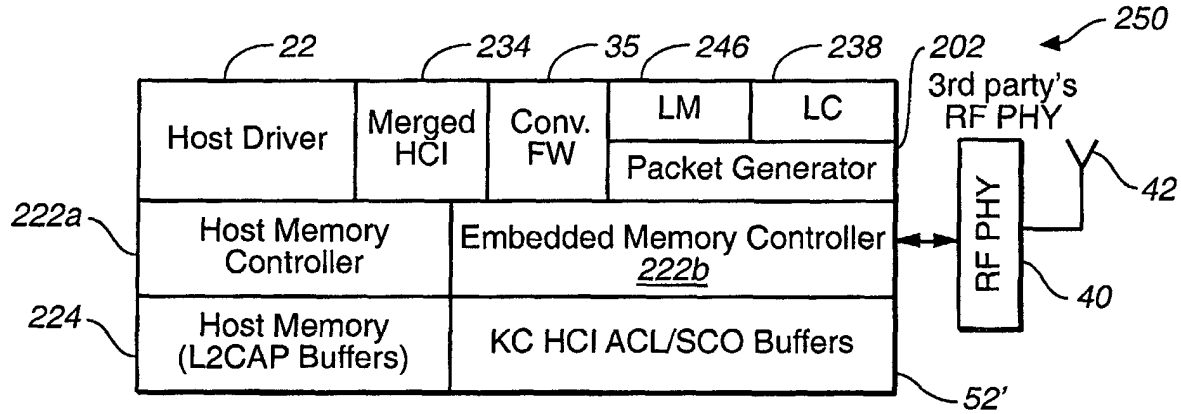
Type A-2: Host / KC Technology Bluetooth BaseBand Controller
