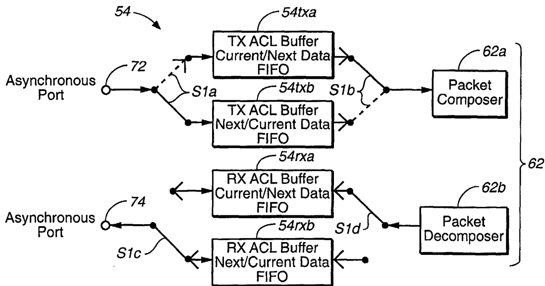
Dual Buffer Scheme For ACL Packet Transmission
