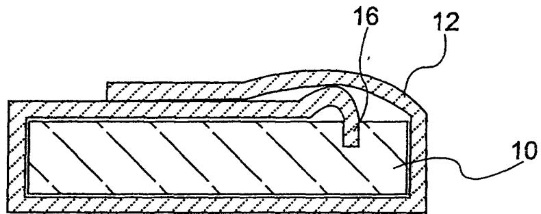
FIG. 3 (RELATED ART)
