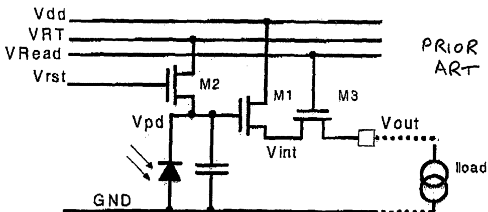
Figure 1 Three Transistor Pixel
