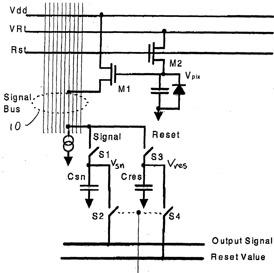
Figure 9 Improved Circuit - Offset Cancellation
