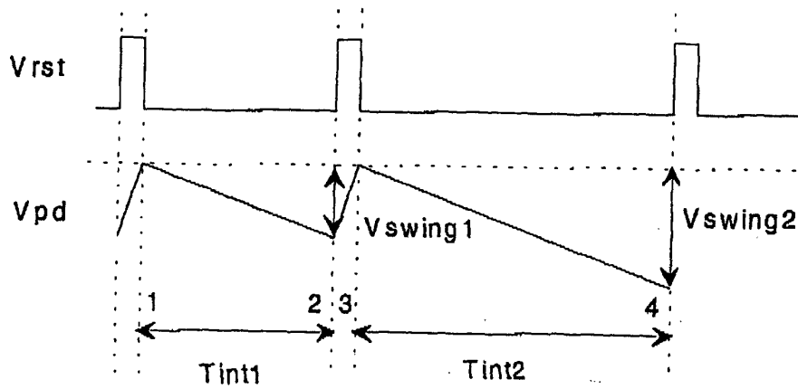
Figure 2 Voltage Swing on Photodiode
