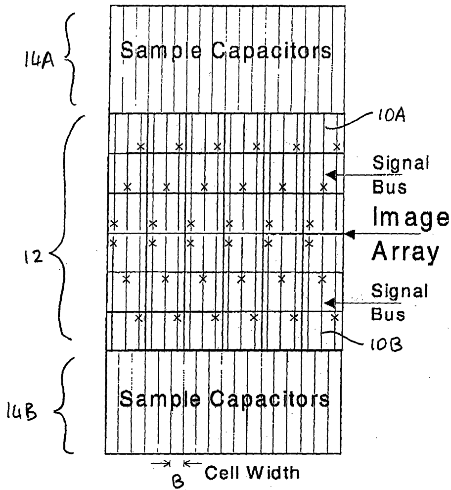
Figure 13 Improved Layout Technique
