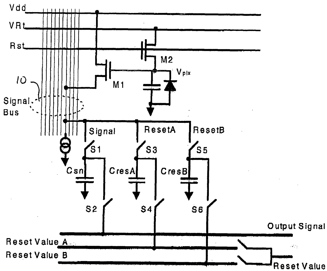
Figure 11 Improved Circuit - Offset Cancellation 2
