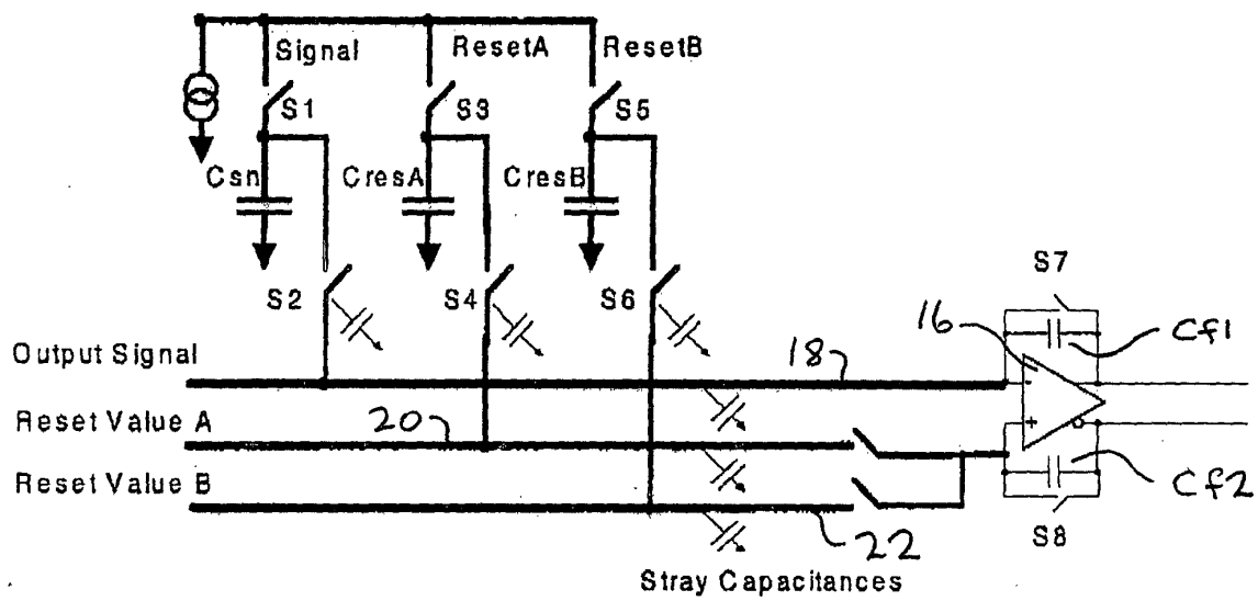
Figure 14 Preferred Readout Amplification
