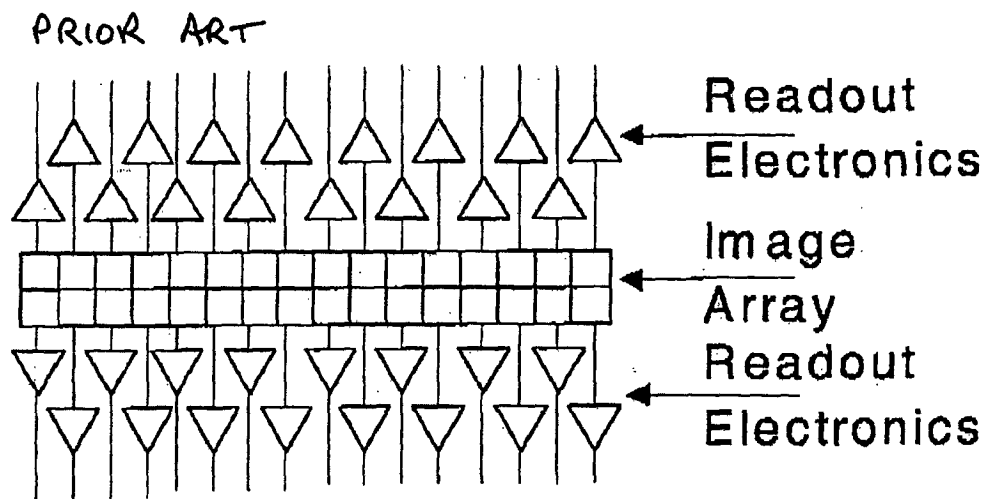
Figure 5 Sophisticated Linear Array
