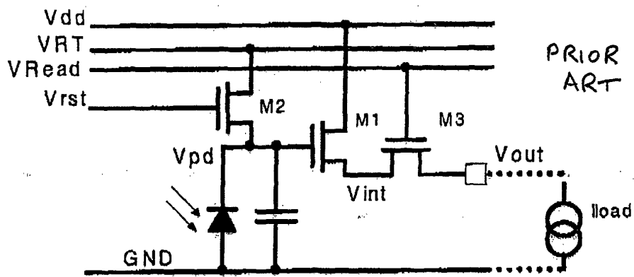
Figure 1 Three Transistor Pixel
