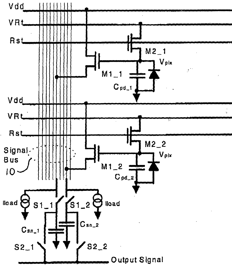
Figure 6 (Part of) New Column Structure
