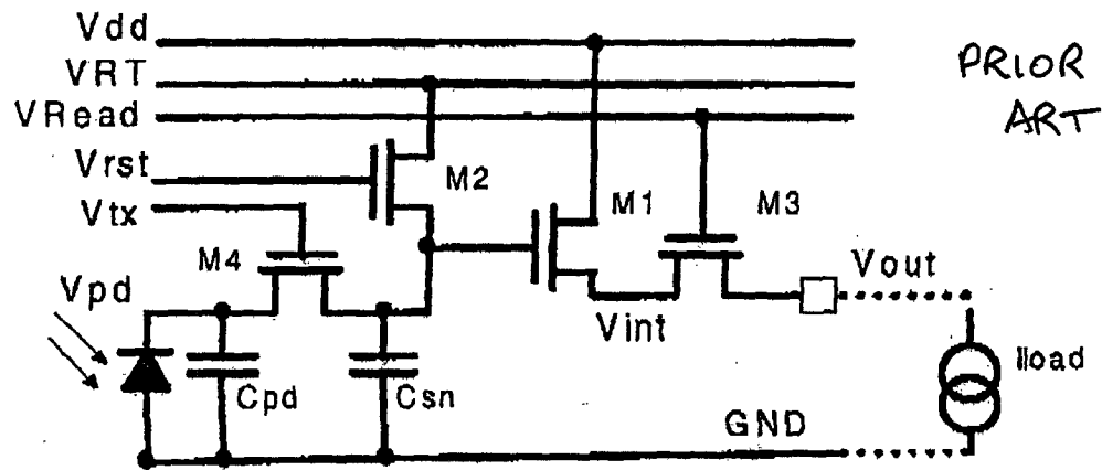
Figure 4 Four Transistor Pixel
