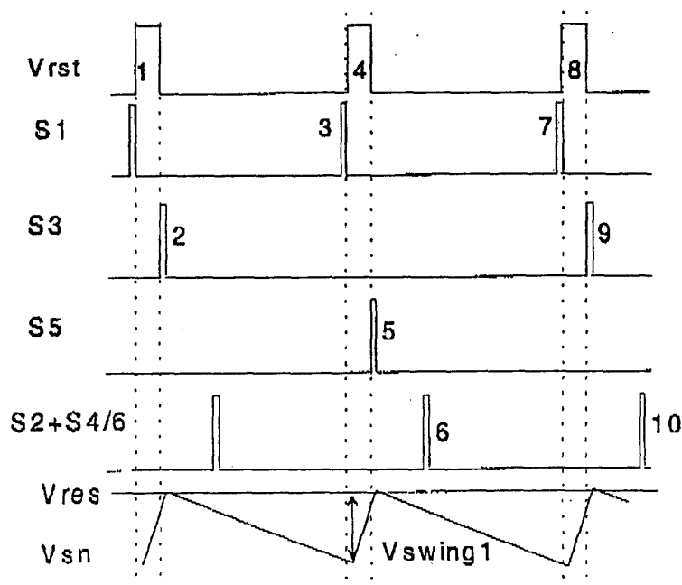
Figure 12 Offset Compensation 2 - Timing Diagram
