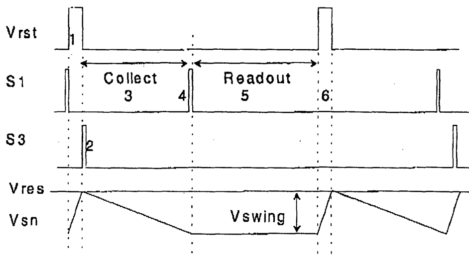
Figure 10 Offset Cancellation - Timing diagram
