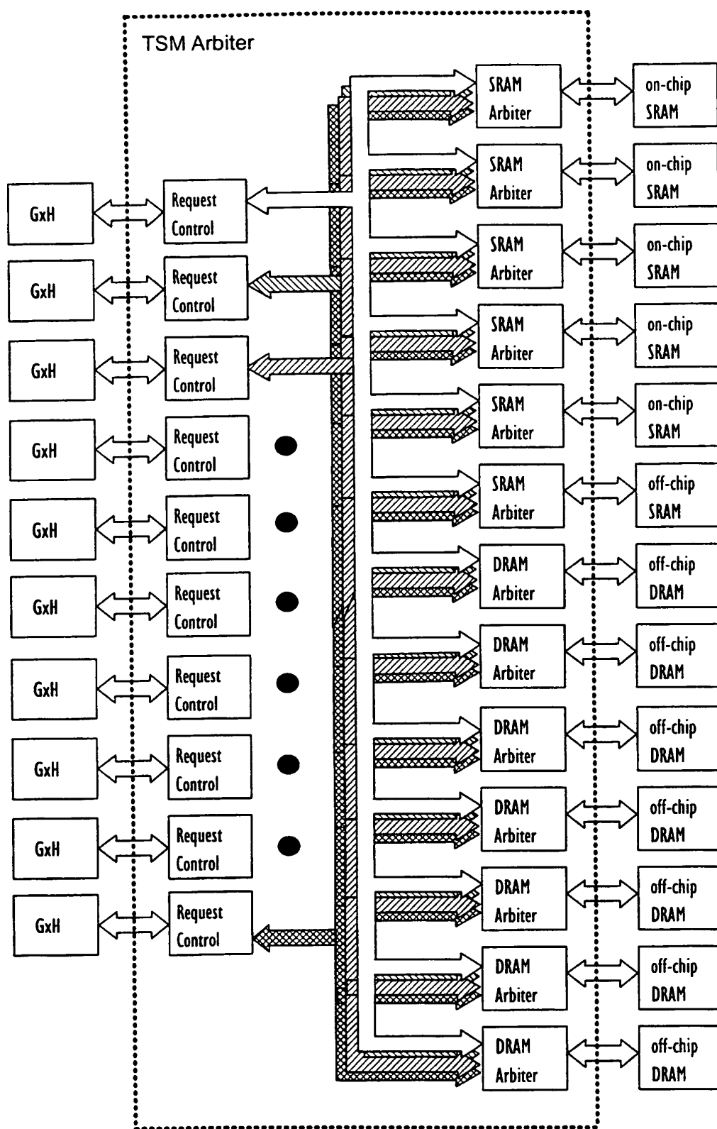
FIG. 13 (Memory Complex)
