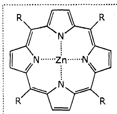
GROOVE BINDING AGENT (Cationic porphyrin)
