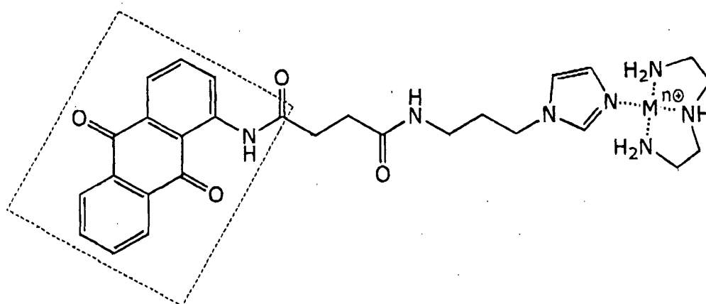
INTERCALATING AGENT (Anthraquinone)
