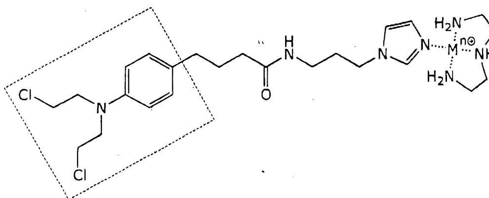
ALKYLATING AGENT (Nitrogen mustard)
