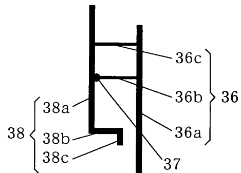
CROSS-SECTIONAL SIDE VIEW FROM ANTENNA-HOUSING BASE PLATE 38
