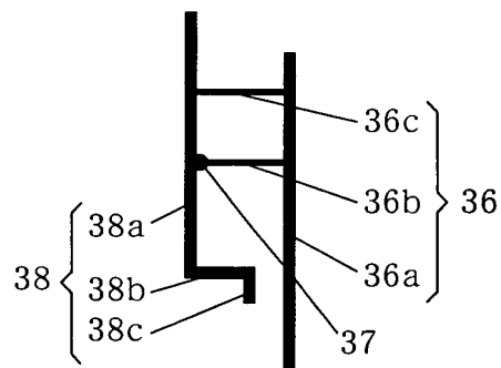
CROSS-SECTIONAL SIDE VIEW FROM ANTENNA-HOUSING BASE PLATE 38
