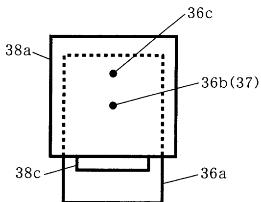
FRONT VIEW FROM ANTENNA-HOUSING BASE PLATE 38
