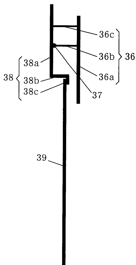
CROSS-SECTIONAL SIDE VIEW OF TWO-CONNECTED BASE PLATES
