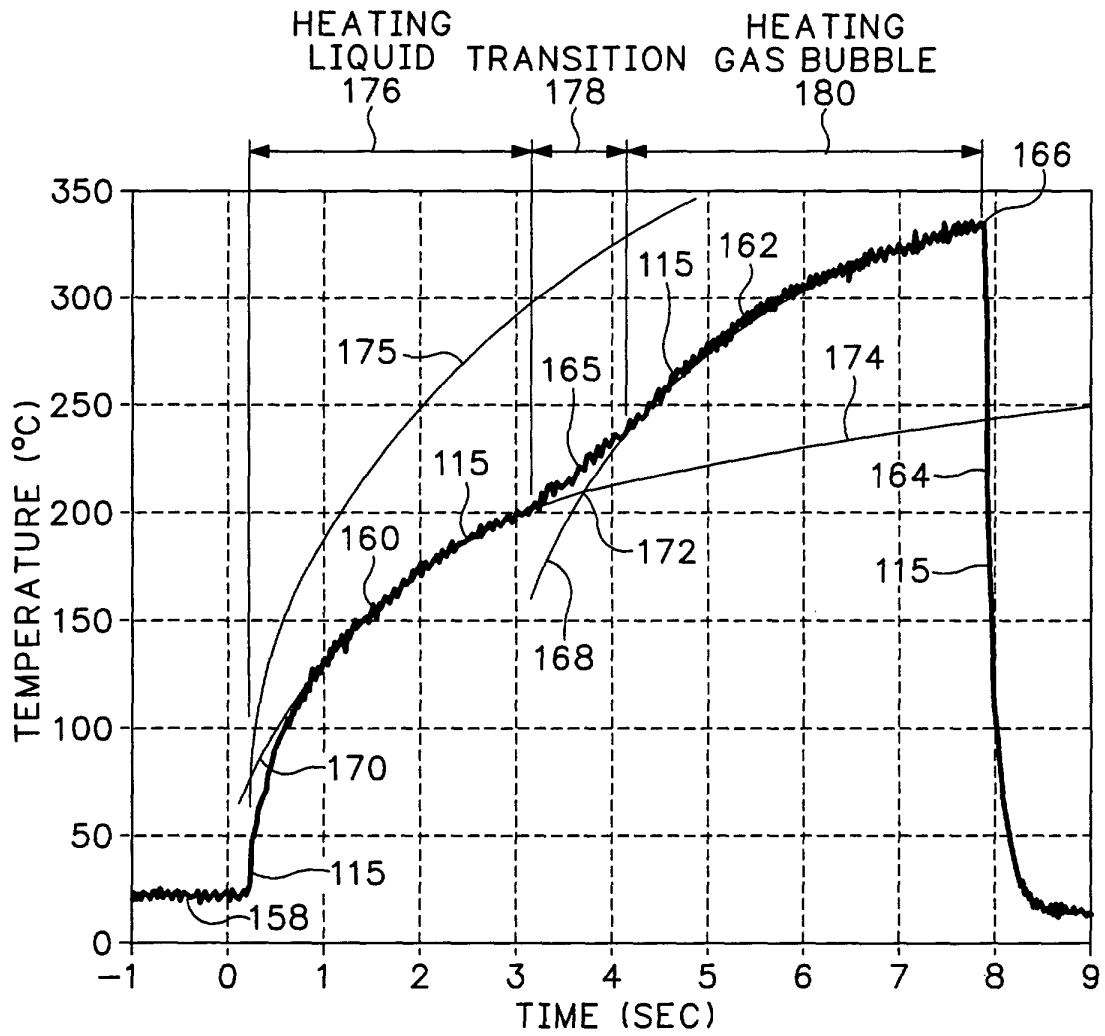
FIRED RESISTOR'S THERMAL CHARACTERISTICS
