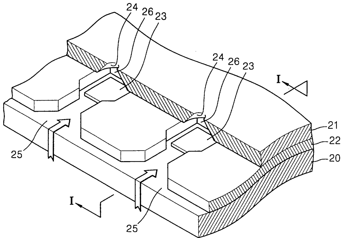
FIG. 2 (PRIOR ART)
