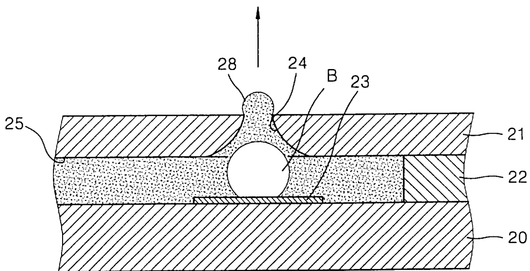
FIG. 3 (PRIOR ART)
