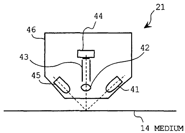
FIG. 4 MEDIUM DETECTION UNIT
