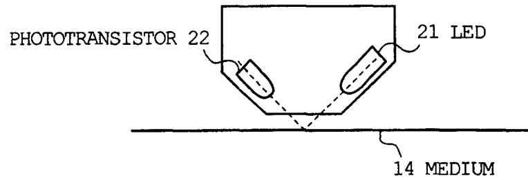
FIG. 3 (a) MEDIUM SENSOR
