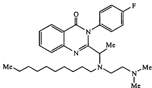
2-[1-(Decyl-(2-dimethylamino-ethyl)-amino)-ethyl]-3-(4-fluoro-phenyl)-3H-quinazolin-4-one (Compound 2.3)
