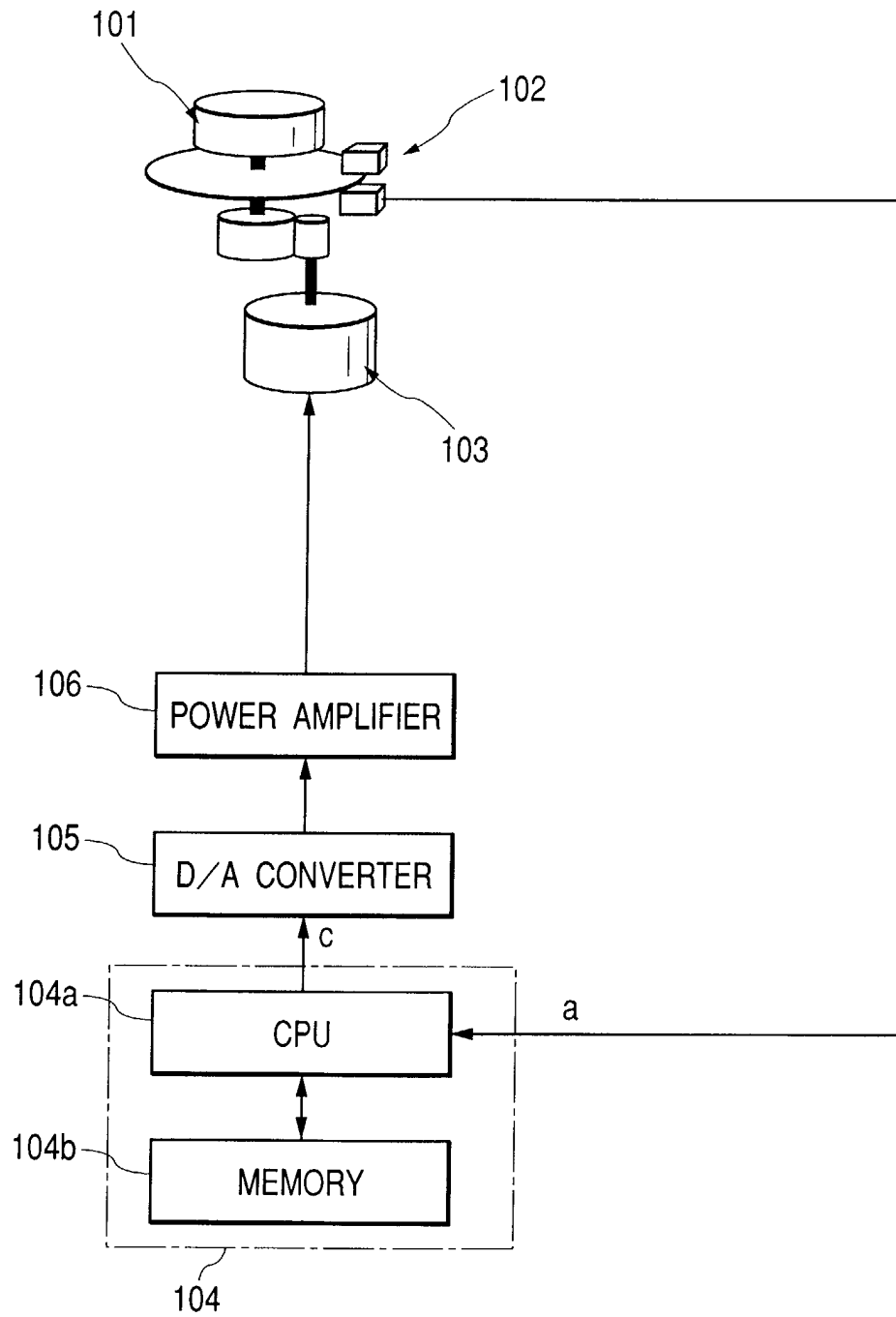
FIG. 10 PRIOR ART
