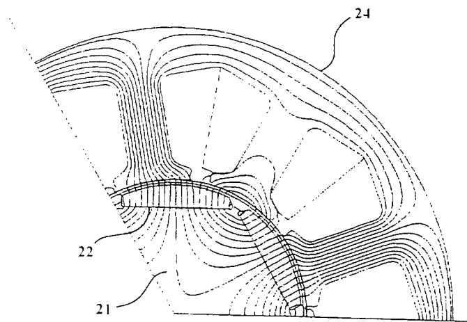
Chart of magnetic flux lines
