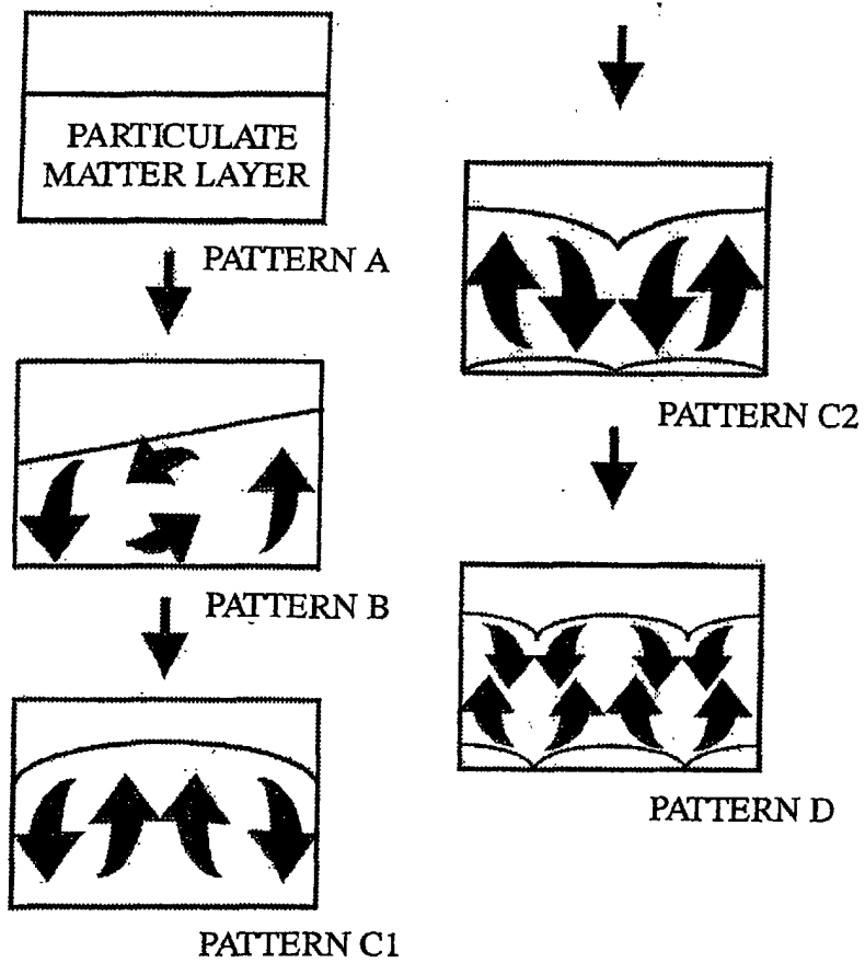
VIBRO-FLUIDIZING PATTERNS (COLORED BEADS, PARTICLE DIAMETER 1mm)
