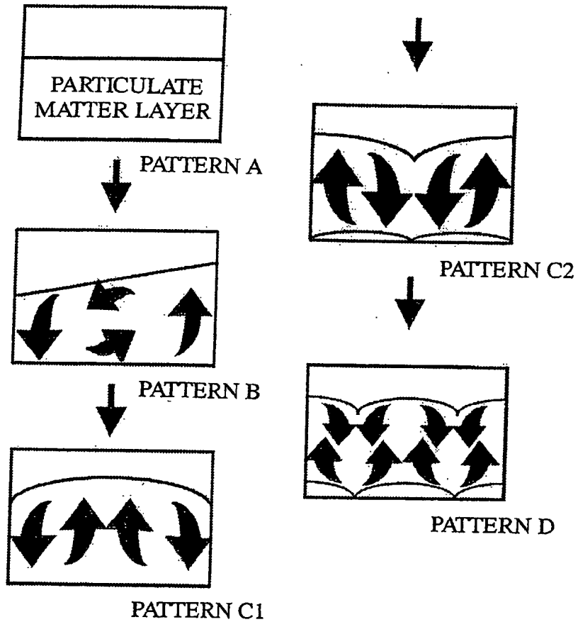
VIBRO-FLUIDIZING PATTERNS (COLORED BEADS, PARTICLE DIAMETER 1mm)
