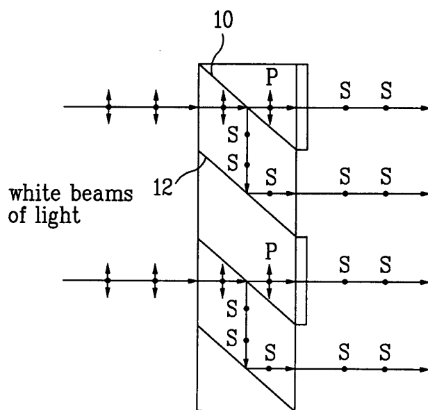
FIG. 2 Background Art
