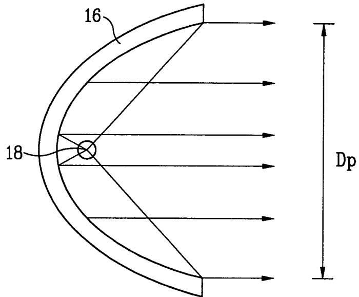
FIG. 4 Background Art
