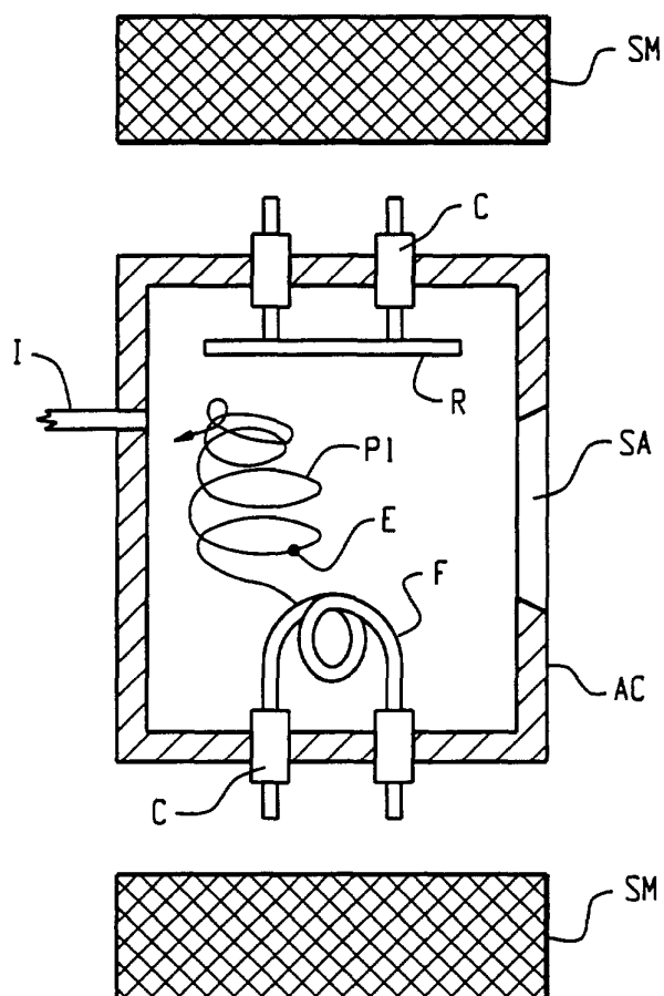
Fig. 1 PRIOR ART
