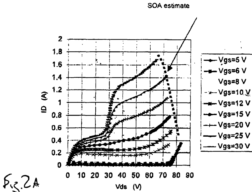
Fig. 2R. Drain characteristic for buried body LDMOS. Pulse measurements with pulse time of 100ns. The approximate location of the SOA boundary is indicated by the dashed line. The increase in ID seen near V_{ds}=30V is an indication that charge compensation due to holes is occurring in the Nwell. W=0.0938 cm.
