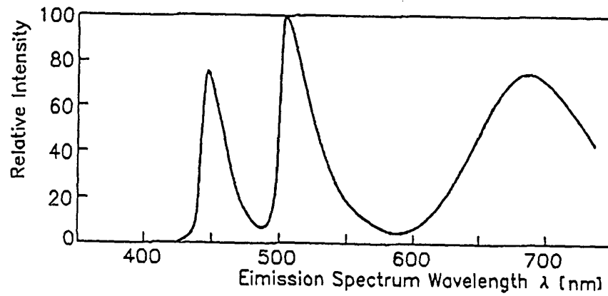
Fig. 1 Emission Spectrum of Light Emitting Device with Light Permeable Fluorescent Cover
