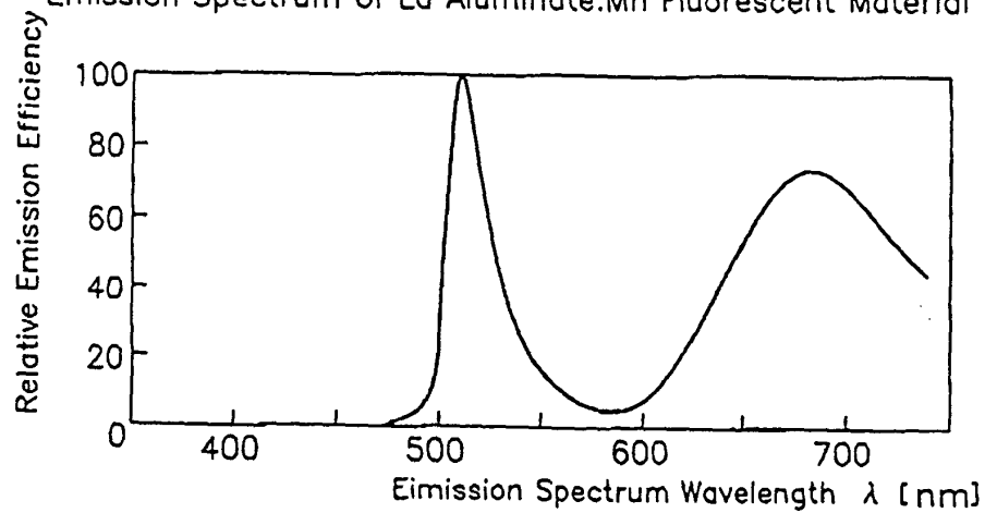
Fig. 3 Emission Spectrum of La Aluminate:Mn Fluorescent Material
