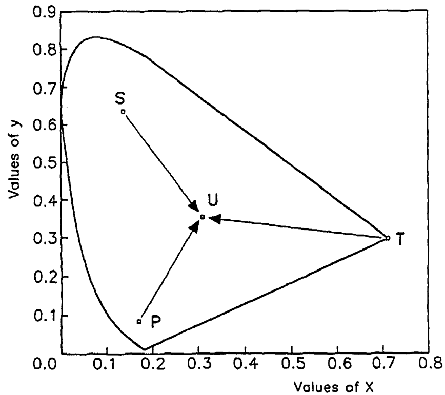
Chromaticity Diagram of Light Emitting Device with La Aluminate:Manganese Fluorescent Material
