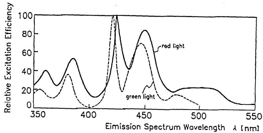
Fig. 2 Excitation Spectrum of La Aluminate:Mn Fluorescent Material
