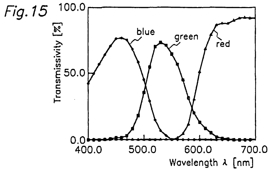
Transmission Spectrum of Color Filter for Transmission Color Liquid Crystal Display
