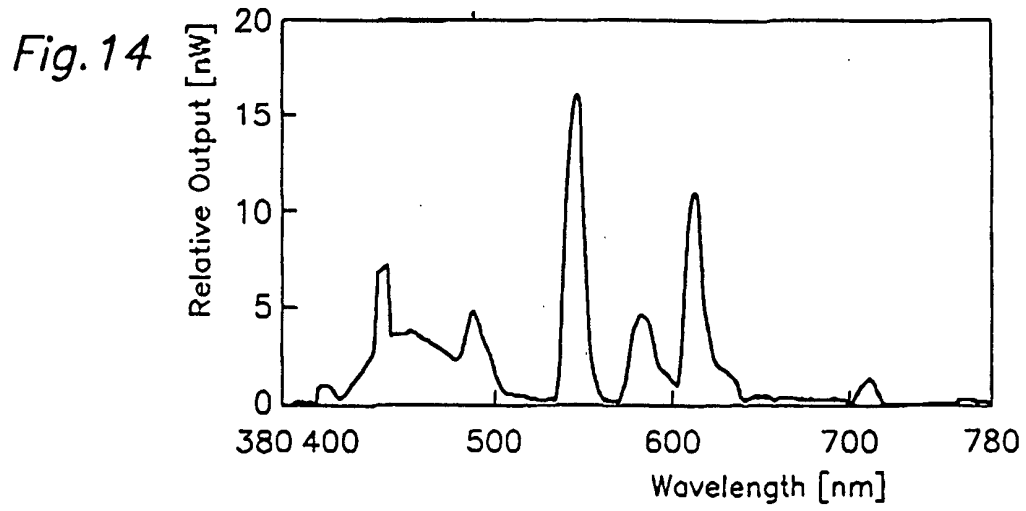
Emission Spectrum of Cold Cathode Fluorescent Tube
