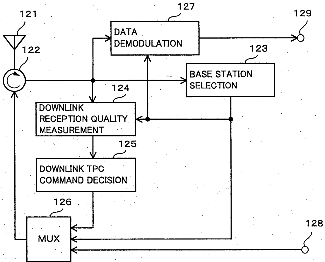
Prior Art Fig. 12
