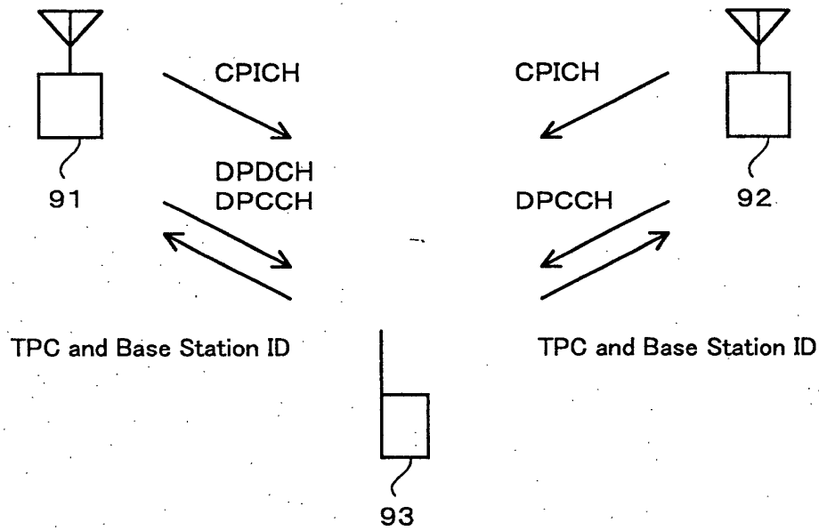
Prior Art Fig. 9
