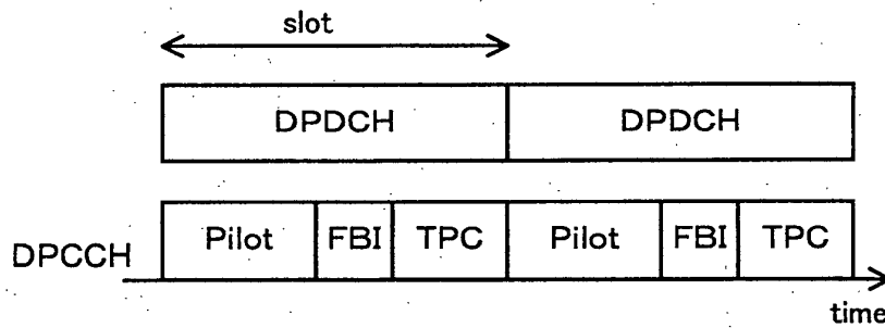
Prior Art Fig. 11
