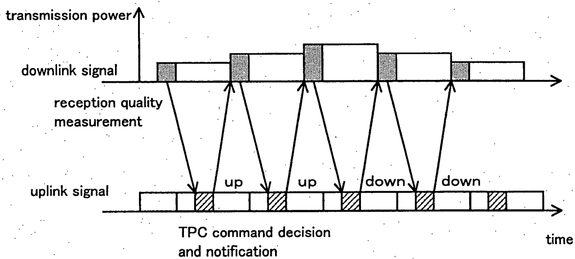
Prior Art Fig. 15
