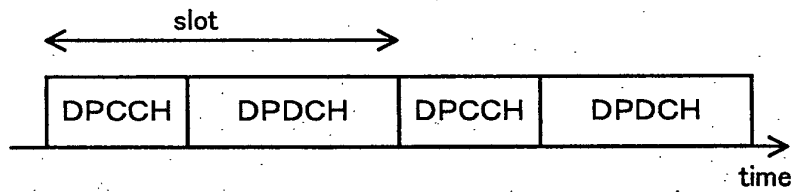
Prior Art Fig. 10
