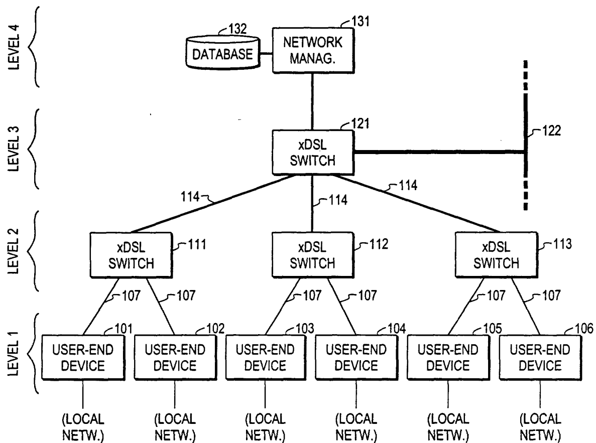
Fig. 1 PRIOR ART
