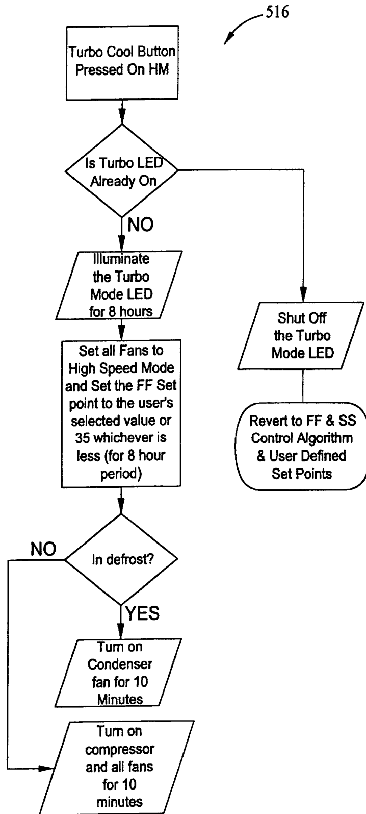
Turbo Cycle Algorithm
