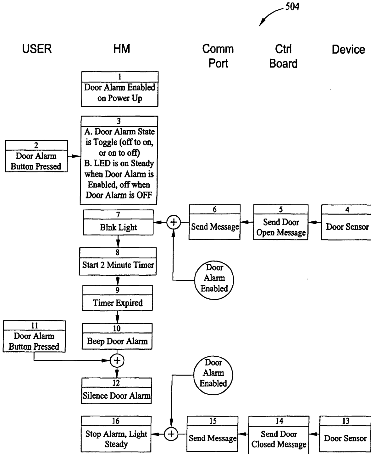
Door Open Interaction Diagram
