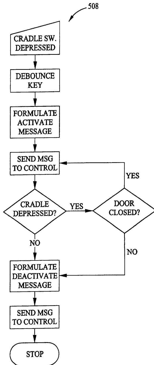
Dispenser Control Algorithm
