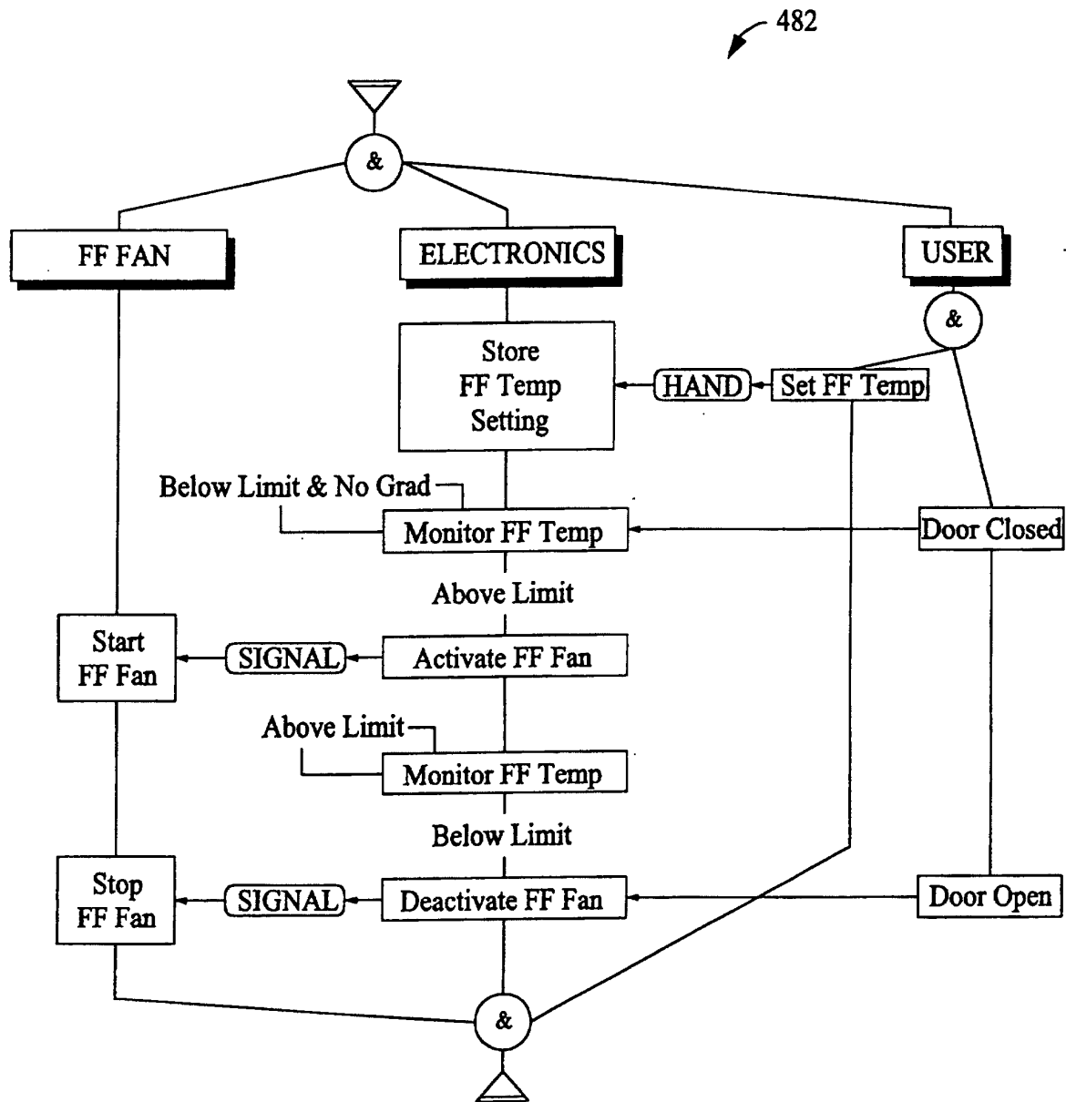
Fresh Food Fan Behavior Diagram
