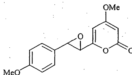
7,8-Epoxyyangonin
