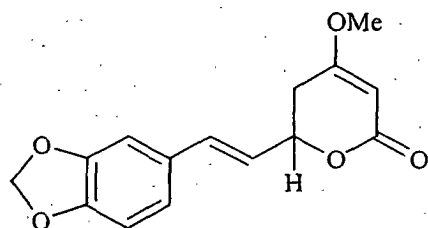
Methysticin
