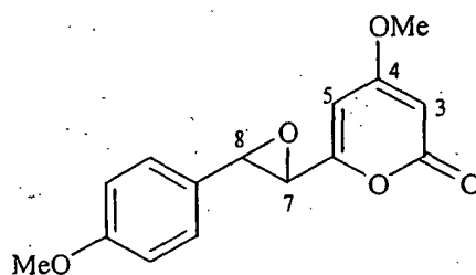
7,8-Epoxyyangonin
