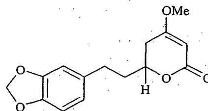
Dihydromethysticin
