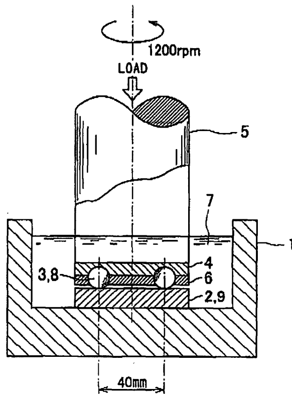
THRUST-TYPE ROLLING ABRATION TESTING MACHINE
