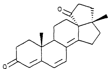
(C-204) [13S,17 \beta ]-3',4'-dihydro-17-methyl-cyclopenta[13,17]-18- norandrost-4,6,8(14)-triene-3,5' [2'H]-dione
