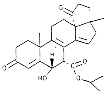
(C-42) 1-methylethyl 3',4',5',17-tetrahydro-6α-hydroxy-17β-methyl-3,5'-dioxocyclopenta[13R,17]-18-norandrost-4,8,14-triene-7α-carboxylate
