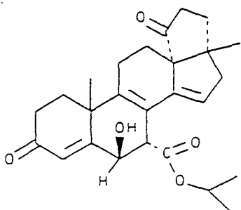
(C-50) 1-methylethyl 3',4',5',17-tetrahydro- 6β-hydroxy-17β-methyl- 3,5'- dioxocyclopenta[13R,17]- 18-norandrosta-4,8,14- triene-7α-carboxylate
