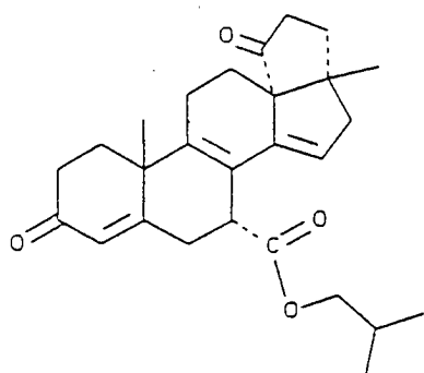
(C-18) 2-methylpropyl 3',4',5',17-tetrahydro- 17β-methyl-3,5'- dioxocyclopenta[13R,17]- 18-norandrost-4,8,14- triene-7α-carboxylate
