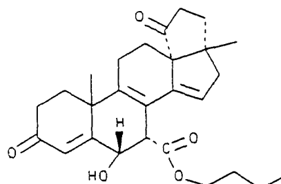
(C-43) butyl 3',4',5',17-tetrahydro-6α-hydroxy-17β-methyl-3,5'-dioxocyclopenta[13R,17]-18-norandrost-4,8,14-triene-7α-carboxylate
