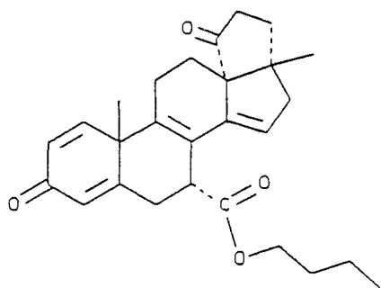
(C-26) butyl 3',4',5',17- tetrahydro-17β-methyl 3,5'- dioxocyclopenta[13R,17]- 18-norandrosta-1,4,8,14- tetraene-7α-carboxylate
