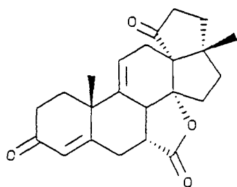
(C-201) (7 \alpha ,13R,17 \beta )-3',4',5',17-tetrahydro-14-hydroxy-17-methyl-3,5'- dioxo- \gamma -lactone, cyclopenta[13,17]-18-norandrost-4,9(11)- diene-7-carboxylic acid
