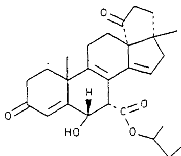
(C-44) 1-methylpropyl 3',4',5',17-tetrahydro- 6 \alpha -hydroxy-17 \beta -methyl- 3,5'- dioxocyclopenta[13R,17]- 18-norandrosta-4,8,14- triene-7 \alpha -carboxylate
