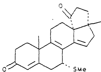
(C-36) 3',4'-dihydro-17-methyl- 7 \alpha -(methylthio)- cyclopenta[13,17]-18- norandrosta-4,8,14- triene-3,5'(2'H)-dione
