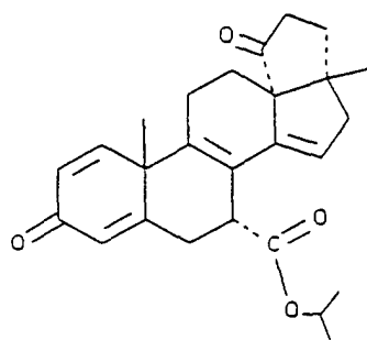
(C-25) 1-methylethyl 3',4',5',17- tetrahydro-17β-methyl-3,5'- dioxocyclopenta[13R,17]-18- norandrosta-1,4,8,14-tetraene- 7α-carboxylate
