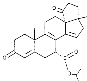
(C-17) 1-methylethyl 3',4',5',17-tetrahydro-17 \beta -methyl-3,5'-dioxocyclopenta[13R,17]-18-norandrost-4,8,14-triene-7 \alpha -carboxylate
