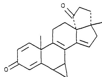
(C-31) 4bR(4bR*),5,5aS*,7,7aR*,8,9, 11,12,12bS*-decahydro-7A,12b- dimethyl-10R*- cyclopropal(1)pentaleno[1,6a- a]phenanthrene-3,10-dione
