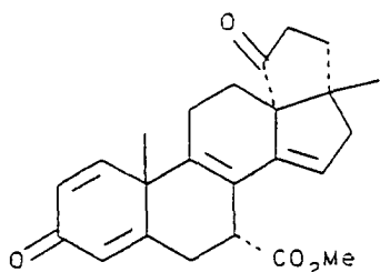
(C-22) methyl 3',4',5',17- tetrahydro-17β-methyl 3,5'- dioxocyclopenta[13R,17]- 18-norandrost-1,4,8,14- tetraene-7α-carboxylate
