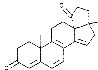
(C-37) 3',4',5,5',6,17-hexahydro-17 \beta - methylcyclopenta[13R,17]-18- norandrosta-4,8,14-triene- 3,5'(2'H)-dione
