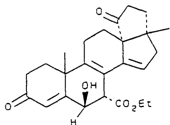
(C-48) ethyl 3',4',5',17- tetrahydro-6 \beta -hydroxy- 17 \beta -methyl-3,5'- dioxocyclopenta[13R,17]- 18-norandrosta-4,8,14- triene-7 \alpha -carboxylate
