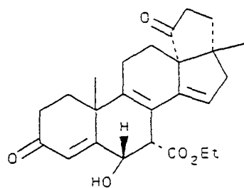
(C-40) ethyl 3',4',5',17-tetrahydro-6α-hydroxy-17β-methyl-3,5'-dioxocyclopenta[13R,17]-18-norandrost-4,8,14-triene-7α-carboxylic acid
