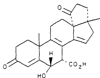
(C-38) 3',4',5',17-tetrahydro- 6 \alpha -hydroxy-17 \beta -methyl- 3,5'- dioxocyclopenta[13R,17]- 18-norandrosta-4,8,14- triene-7 \alpha -carboxylic acid
