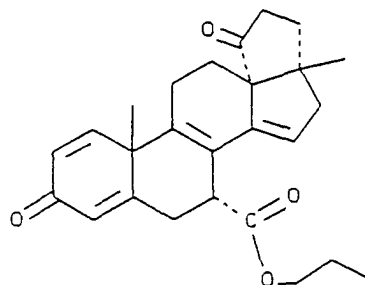
(C-23) propyl 3',4',5',17-tetrahydro- 17β-methyl-3,5'- dioxocyclopenta[13R,17]-18- norandrost-1,4,8,14-tetraene- 7α-carboxylate
