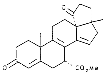
(C-1) methyl 2,2,3a,4,6,7,9, 10,11,11a,12,13-dodecahydro- 3αβ,11αβ-dimethyl-1,9-dioxo- 1H-pentaleno[1,6a- a]phenantrene-6α-carboxylate
