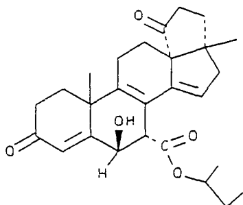
(C-52) 1-methylpropyl 3',4',5',17-tetrahydro- 6β-hydroxy-17β-methyl- 3,5'- dioxocyclopenta[13R,17]- 18-norandrosta-4,8,14- triene-7α-carboxylate
