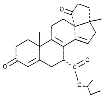
(C-19) 1-methylpropyl 3',4',5',17- tetrahydro-17β-methyl-3,5'- dioxocyclopenta[13R,17]-18- norandrost-4,8,14-triene-7α- carboxylate
