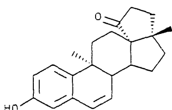
(C-203) [13S,17 \beta ]-3',4'-dihydro-3-hydroxy-9,17- dimethylcyclopenta[13,17]gona-1,3,5(10),6-tetraene-5' [2'H]-one
