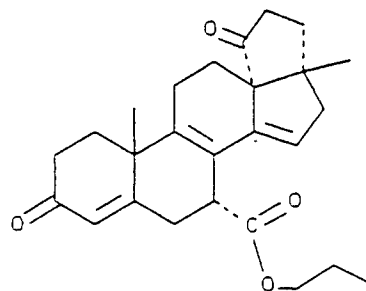
(C-15) propyl 3',4',5',17-tetrahydro-17 \beta -methyl-3,5'-dioxocyclopenta[13R,17]-18-norandrost-4,8,14-triene-7 \alpha -carboxylate
