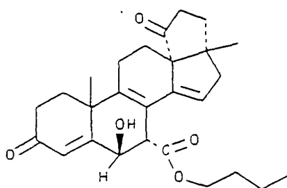
(C-53) butyl 3',4',5',17- tetrahydro-6β-hydroxy- 17β-methyl-3,5'- dioxocyclopenta[13R,17]- 18-norandrosta-4,8,14- triene-7α-carboxylate
