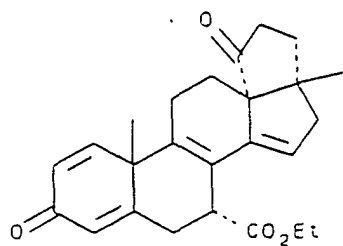
(C-24) ethyl 3',4',5',17- tetrahydro-17β-methyl 3,5'- dioxocyclopenta[13R,17]- 18-norandrosta-1,4,8,14- tetraene-7α-carboxylate
