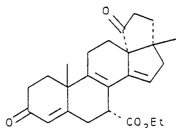
(C-14) ethyl 3',4',5',17-tetrahydro-17 \beta -methyl-3,5'-dioxocyclopenta[13R,17]-18-norandrost-4,8,14-triene-7 \alpha -carboxylate
