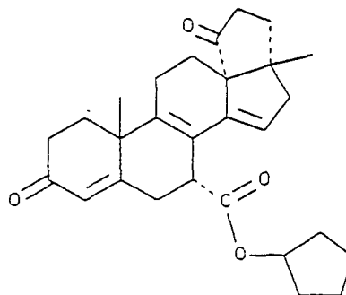
(C-51) cyclopentyl 3',4',5',17- tetrahydro-17β-methyl 3,5'- dioxocyclopenta[13R,17]-18- norandrosta-4,8,14-triene-7α- carboxylate
