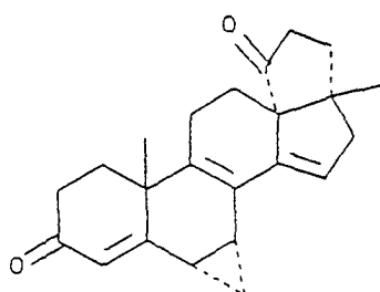
(C-32) 1,2,4bS(4bR*),5,5aS*,8,9, 11,12,12bR*-dodecahydro- 7a,12b-dimethyl-10aS*-cy- clopropal[1]pentaleno[1, 6a-a]phenanthrene-3,10- dione
