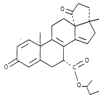
(C-27) 1-methylpropyl 3',4',5',17- tetrahydro-17β-methyl-3,5'- dioxocyclopenta[13R,17]-18- norandrosta-1,4,8,14-tetraene- 7α-carboxylate
