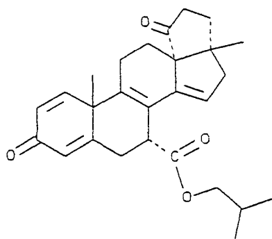
(C-28) 2-methylpropyl 3',4',5',17-tetrahydro- 17 \beta -methyl 3,5'- dioxocyclopenta[13R,17]- 18-norandrost-1,4,8,14- tetraene-7 \alpha -carboxylate
