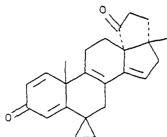
(C-33) 2',3',3'a \alpha ,4',6',11'a \alpha ,12',13' -octahydro-3'aR,3'a,11'a- dimethyl-13'aR*- spiro[cyclopropane-1,7'(9'H)- [1H]pentaleno[1,6,a- a]phenanthrene]-1',9'-dione
