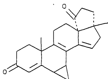
(C-30) 1,2,4bR(4bR*),5,5aS*,7, 7aR*,8,9,11,12bS*- dodecahydro-7a,12b- dimethyl-10aR*-cyclo- propal[1]pentaleno[1,6a- a]phenanthrene-3,10-dione
