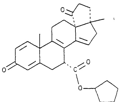
(C-20) cyclopentyl 3',4',5',17- tetrahydro-17β-methyl- 3,5'- dioxocyclopenta[13R,17]- 18-norandrost- 1,4,8,14-tetraene-7α- carboxylate
