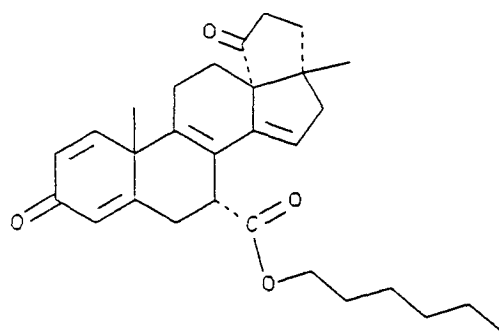
(C-29) hexyl 3',4',5',17-tetrahydro- 17 \beta -methyl-3,5'- dioxocyclopenta[13R,17]-18- norandrost-1,4,8,14-tetraene- 7 \alpha -carboxylate
