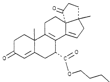
(C-16) butyl 3',4',5',17-tetrahydro-17 \beta -methyl-3,5'-dioxocyclopenta[13R,17]-18-norandrost-4,8,14-triene-7 \alpha -carboxylate
