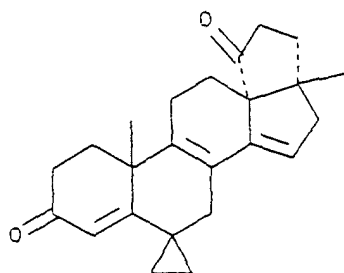
(C-34) 2',3',3'a \alpha ,4',6',10',11', 11'a \alpha ,12',13'-decahydro- 3'aR,3'a,11'a-dimethyl- 13'aR*- spiro[cyclopropane- 1,7'(9'H)- [1H]pentaleno[1,6a-a] phenanthrene]-1',9'-dione
