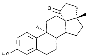
(C-202) [13S,17 \beta ]-3',4'-dihydro-3-hydroxy-9,17- dimethylcyclopenta[13,17]gona-1,3,5(10)-triene-5' [2'H]-one
