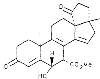
(C-39) methyl 3',4',5',17-tetrahydro- 6 \alpha -hydroxy-17 \beta -methyl-3,5'- dioxocyclopenta[13R,17]-18- norandrosta-4,8,14-triene-7 \alpha - carboxylate
