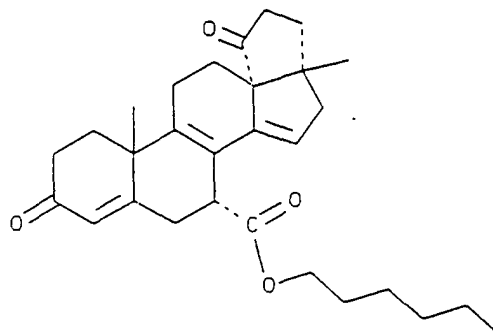
(C-21) hexyl 3',4',5',17-tetrahydro- 17β-methyl-3,5'- dioxocyclopenta[13R,17]-18- norandrost-4,8,14-triene-7α- carboxylate
