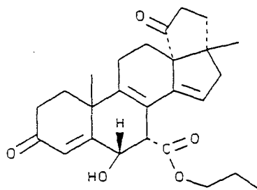
(C-41) propyl 3',4',5',17-tetrahydro-6α-hydroxy-17β-methyl-3,5'-dioxocyclopenta[13R,17]-18-norandrost-4,8,14-triene-7α-carboxylate
