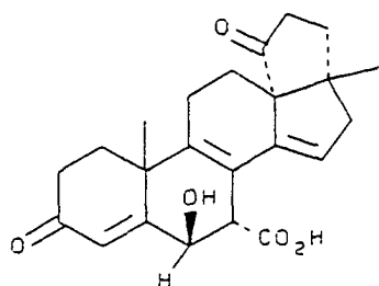
(C-46) 3',4',5',17-tetrahydro- 6 \beta -hydroxy-17 \beta -methyl- 3,5'- dioxocyclopenta[13R,17]- 18-norandrosta-4,8,14- triene-7 \alpha -carboxylic acid
