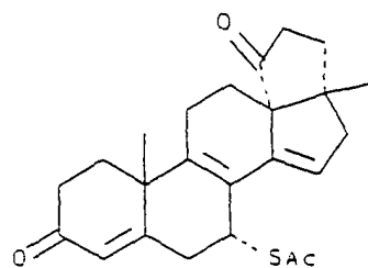
(C-35) 7 \alpha -(acetylthio)-3',4'-dihydro- 17-methyl-cyclopenta[13,17]- 18-norandrosta-4,8,14-triene- 3,5'(2'H)-dione
