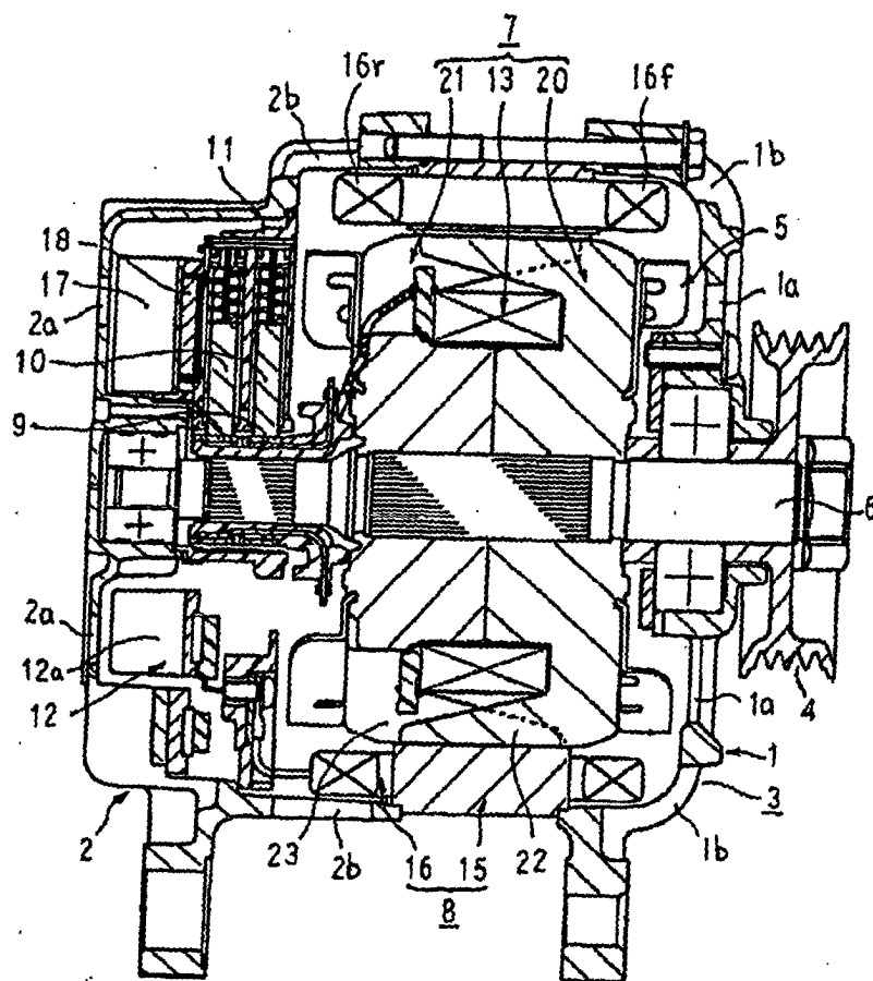
FIG. 22 PRIOR ART
