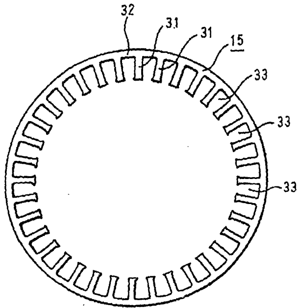
FIG. 25 PRIOR ART
