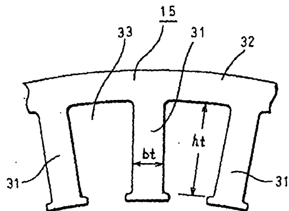
FIG. 26 PRIOR ART
