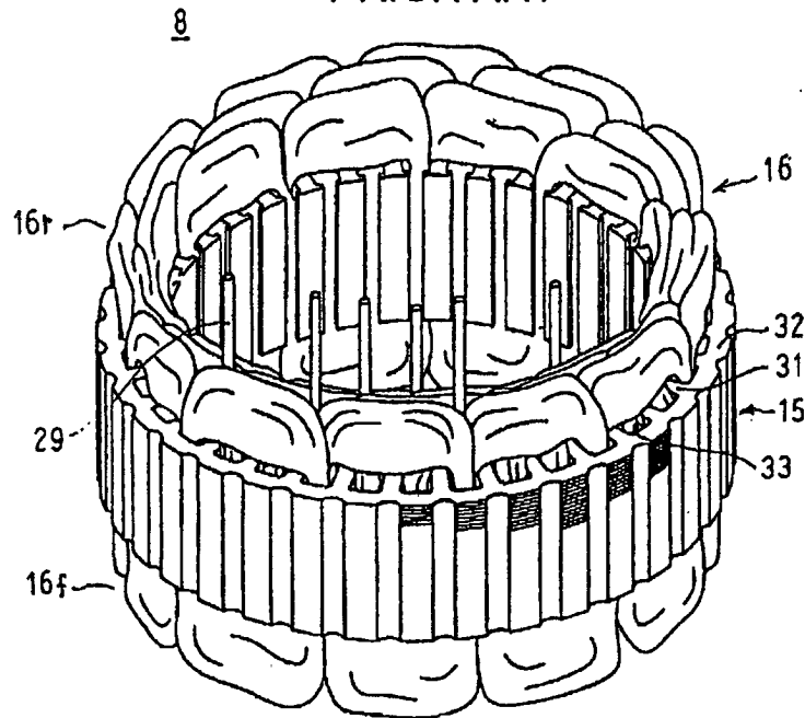
FIG. 23 PRIOR ART
