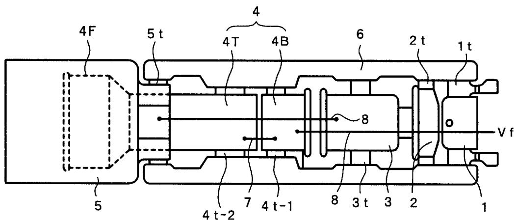
FIG. 14 (Prior Art)
