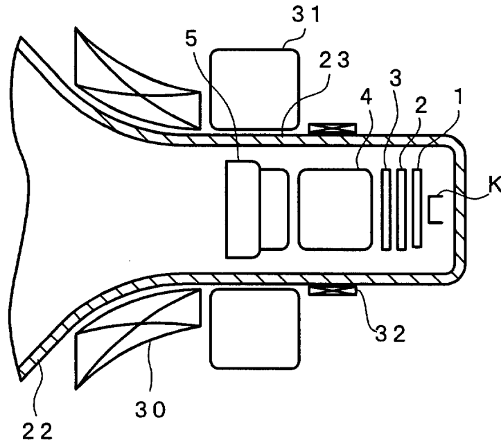
FIG. 13 (Prior Art)
