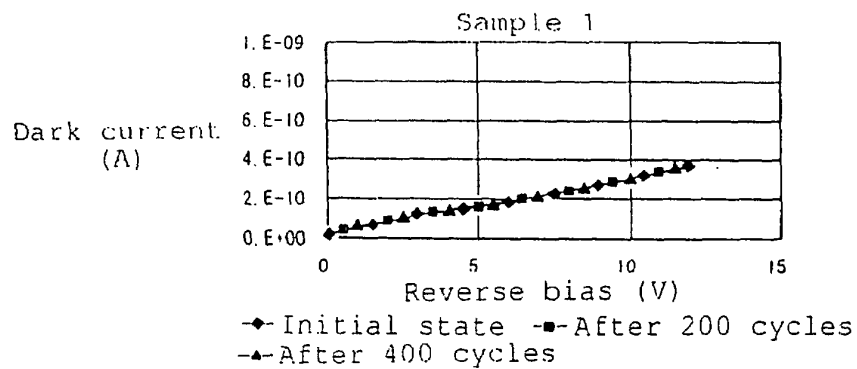
FIG. 2C-2 Temperature cycle test (-40 to 125 °C)
