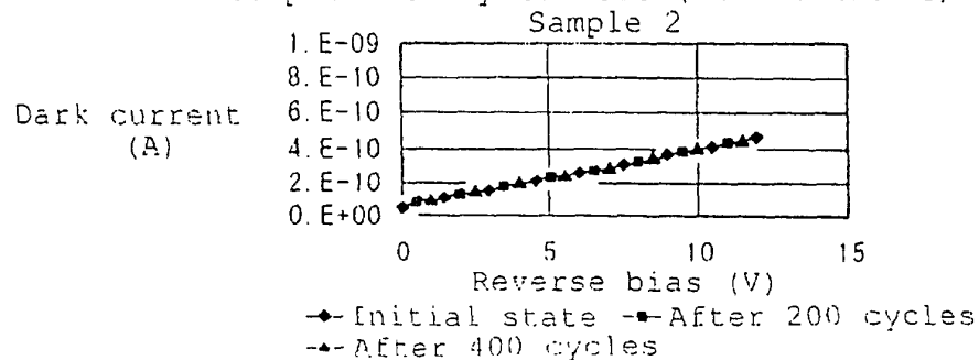
FIG. 2C-2 Temperature cycle test (-40 to 125 °C)
