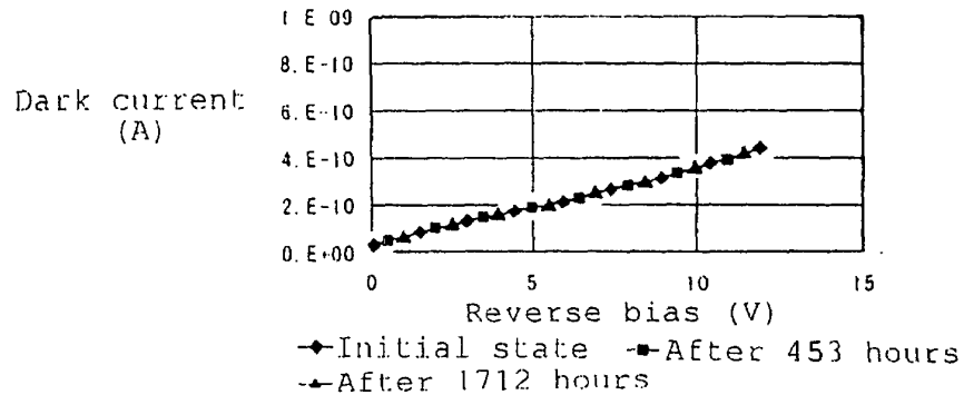
FIG. 2C-1 Temperature cycle test (-40 to 125 °C)
