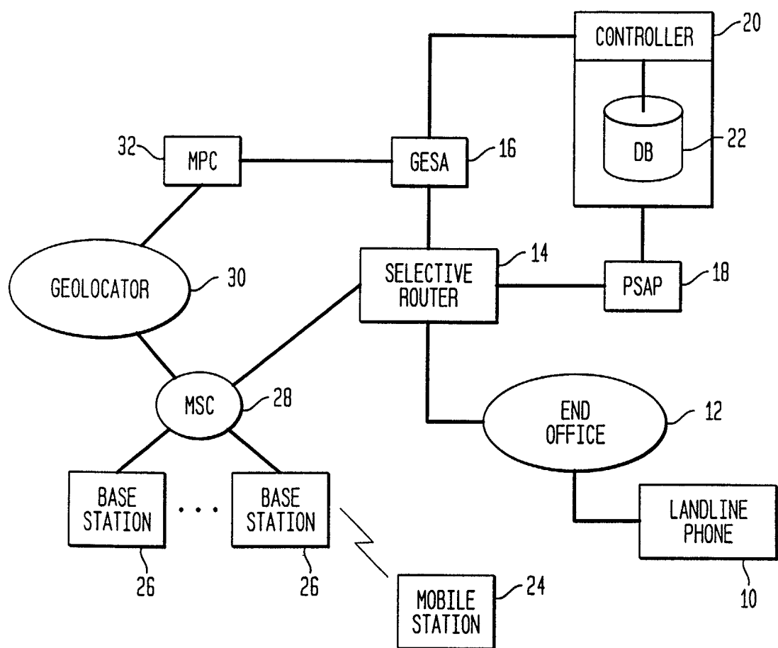
FIG. 1 (PRIOR ART)
