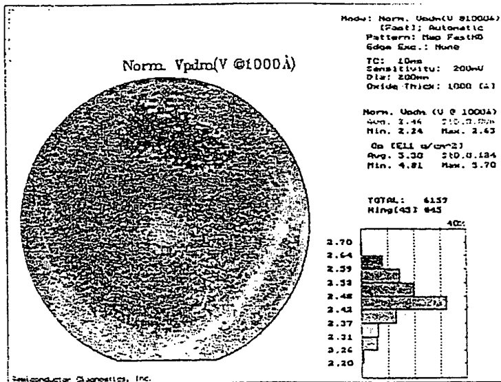
Fig. 8(b) Edge-fast Deposition
