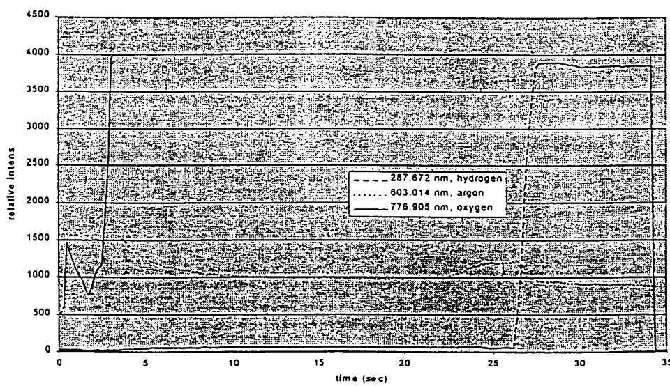
Fig. 9 (b) Center-fast deposition
