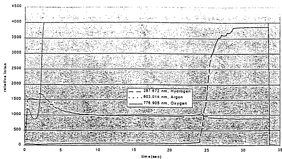
Fig. 9(a) Edge-fast deposition
