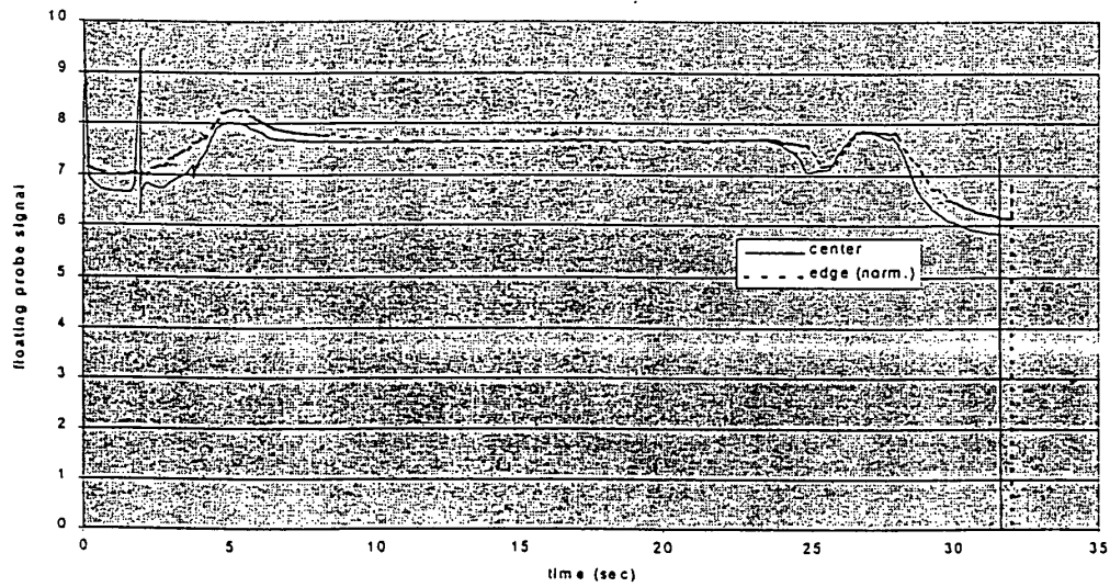
Fig. 10(b) Center-fast Deposition
