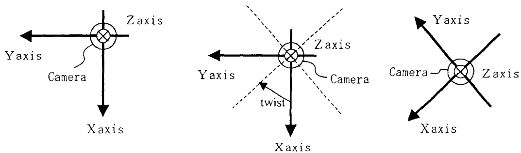
FIG. 6C Setting of the twist around the optical axis of the camera
