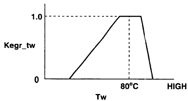
TARGET EGR RATIO CORRECTION TABLE
