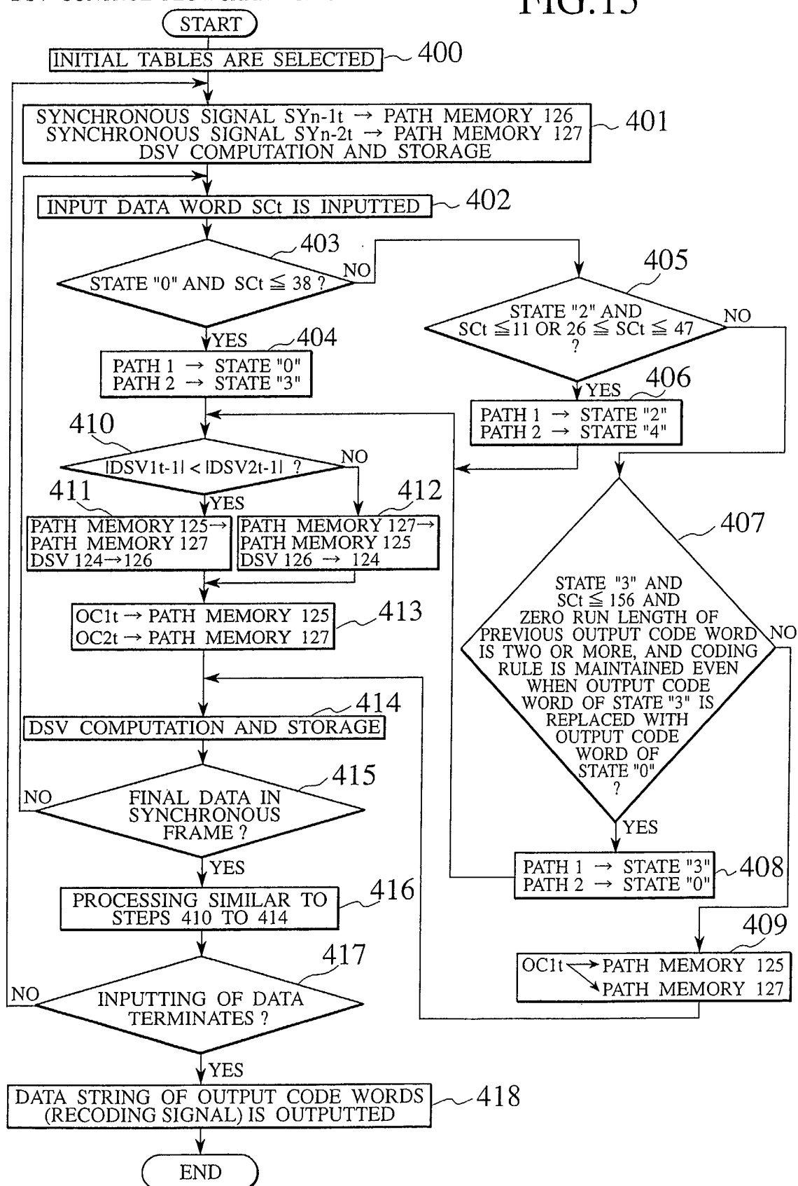
DSV CONTROL FLOWCHART OF 8-15 MODULATION FIG.15
