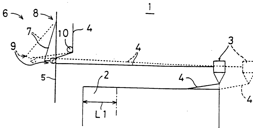
FIG. 25 PRIOR ART
