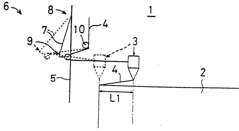
FIG. 24 PRIOR ART
