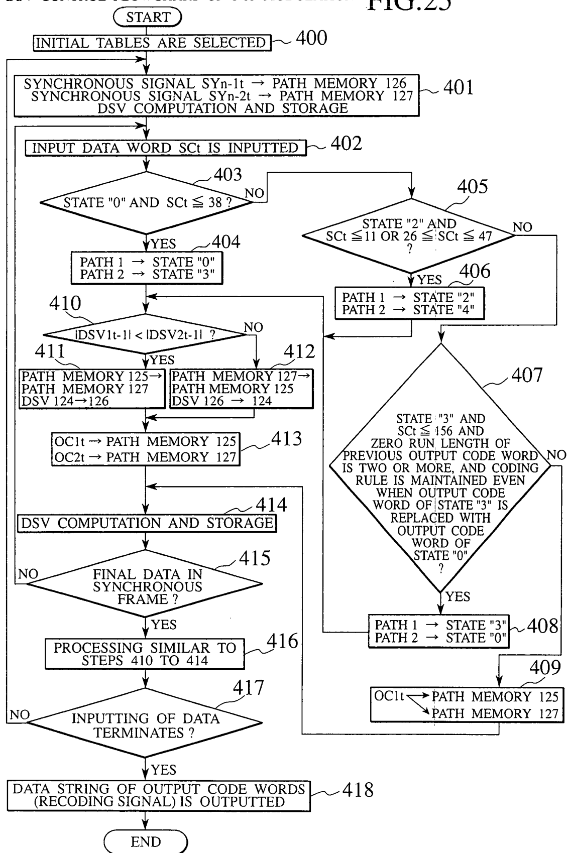
DSV CONTROL FLOWCHART OF 8-15 MODULATION FIG.25
