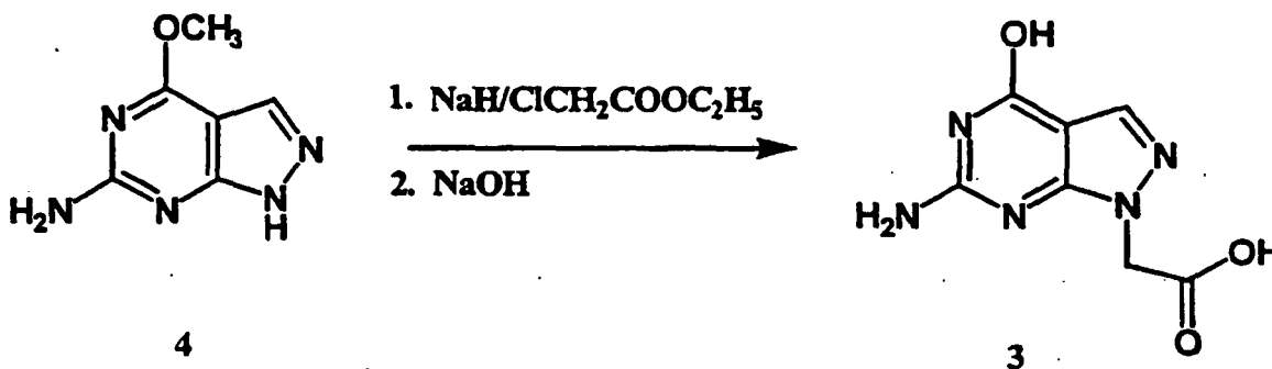
Reaction Scheme 1
