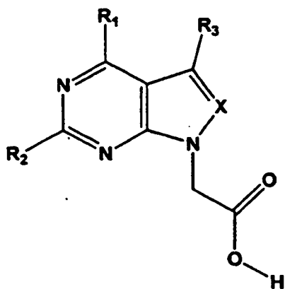
Formula 2
