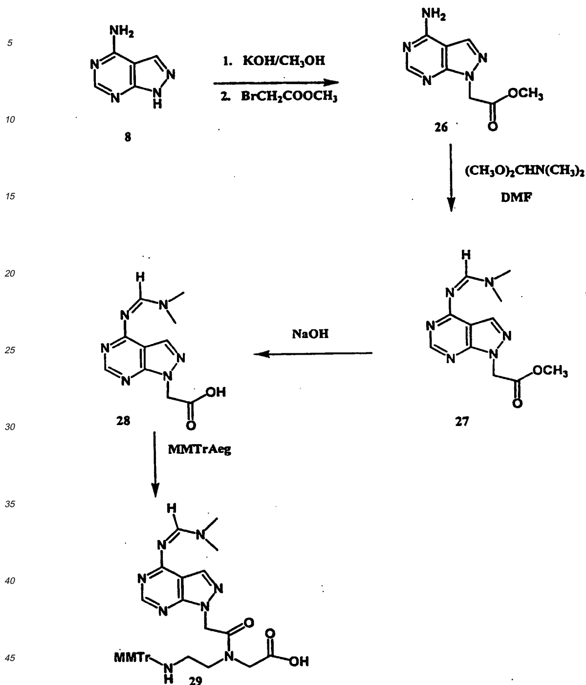
Reaction Scheme 8
