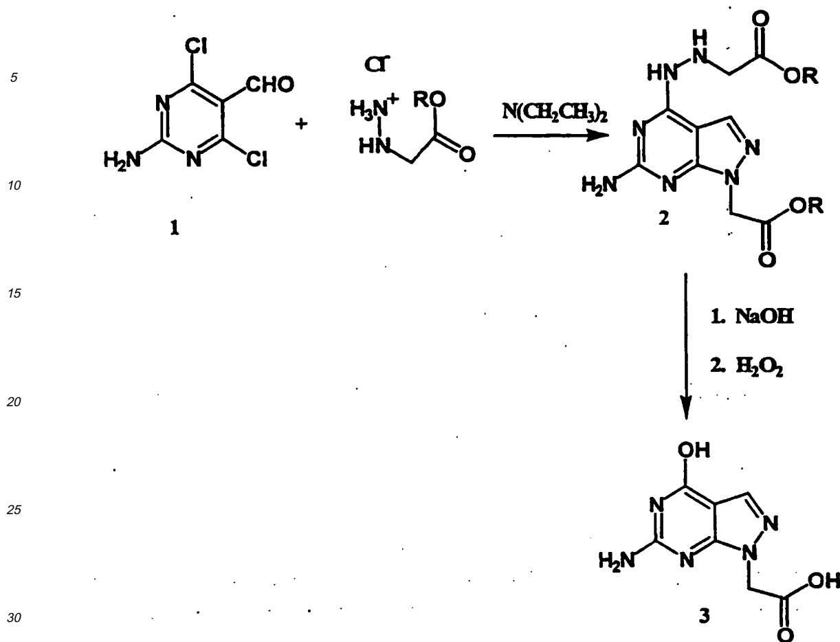
Reaction Scheme 2
