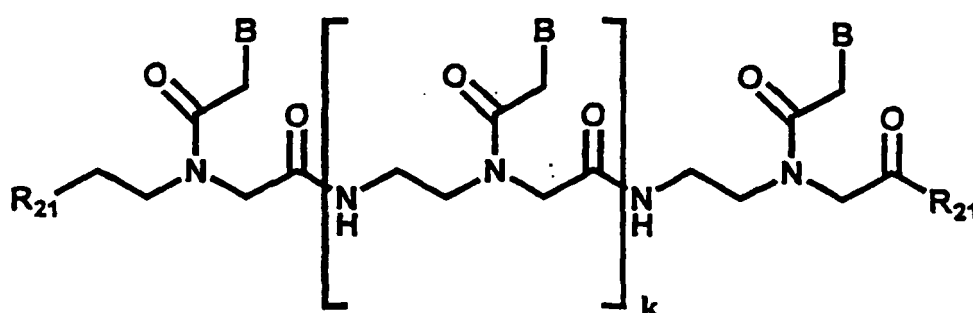
Formula 4
