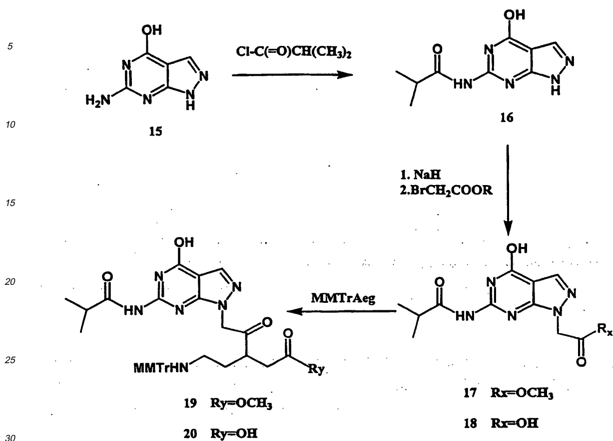
Reaction Scheme 5
