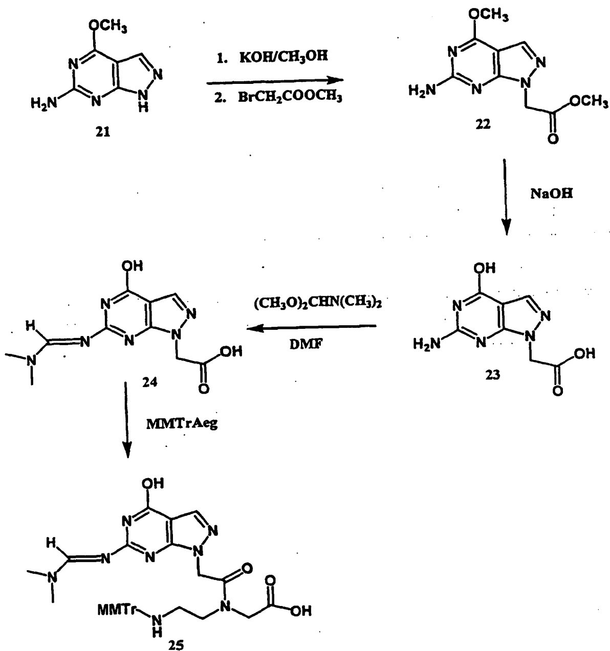
Reaction Scheme 7
