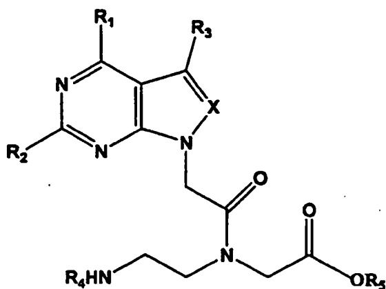
Formula 3
