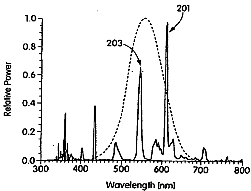
Fig. 27 (Prior Art)
