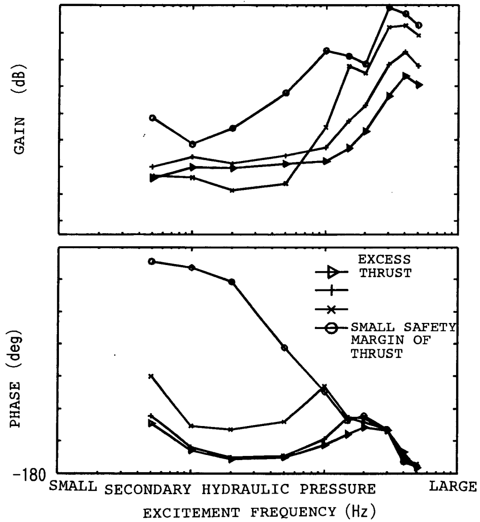
HYDRAULIC PRESSURE-THRUST RATIO TRANSMISSION CHARACTERISTICS
