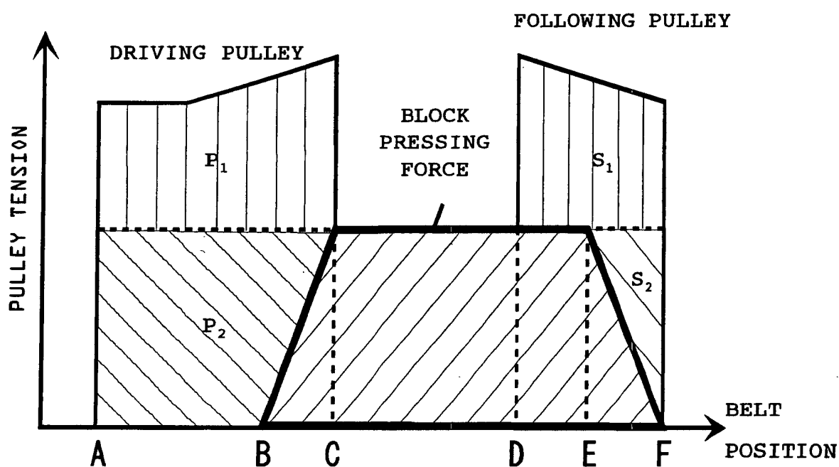
THRUST RATIO IN CASE WITH EXCESS THRUST
