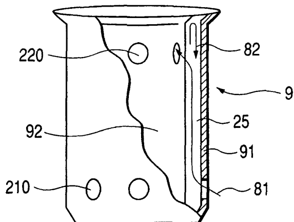
FIG. 16 PRIOR ART
