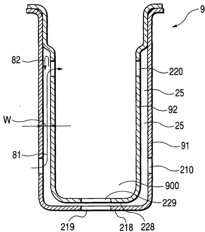
FIG. 17 PRIOR ART
