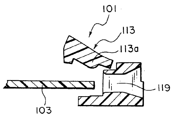
FIG. 13 PRIOR ART
