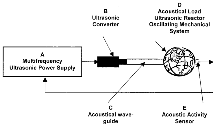
Fig. 1 Block Diagram of a Multifrequency Structural Actuator
