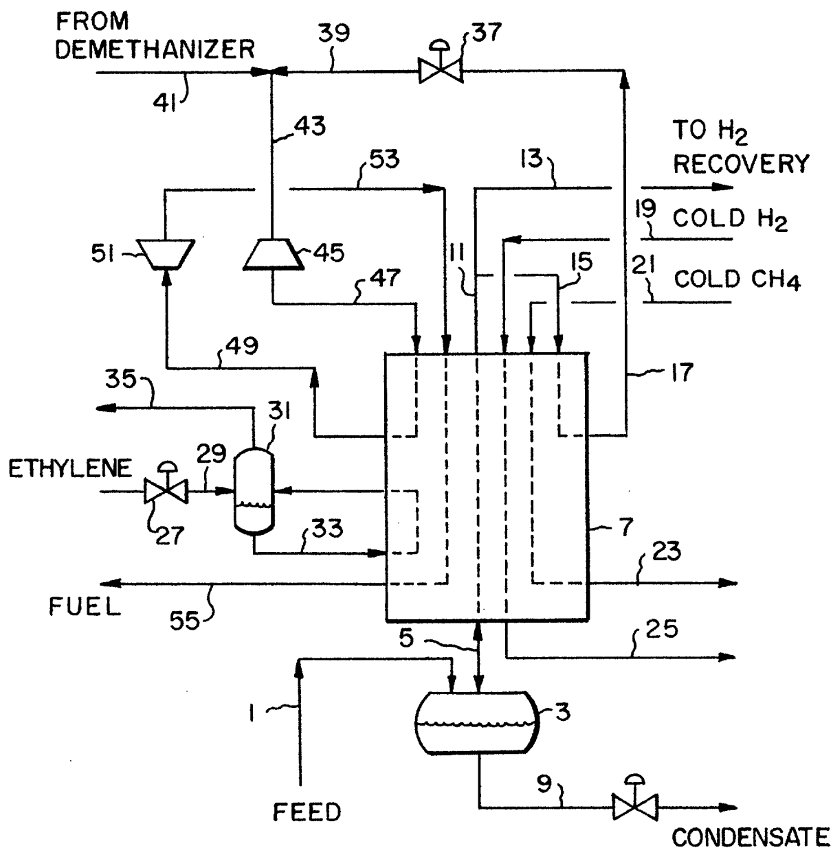
FIG. 1 (PRIOR ART)
