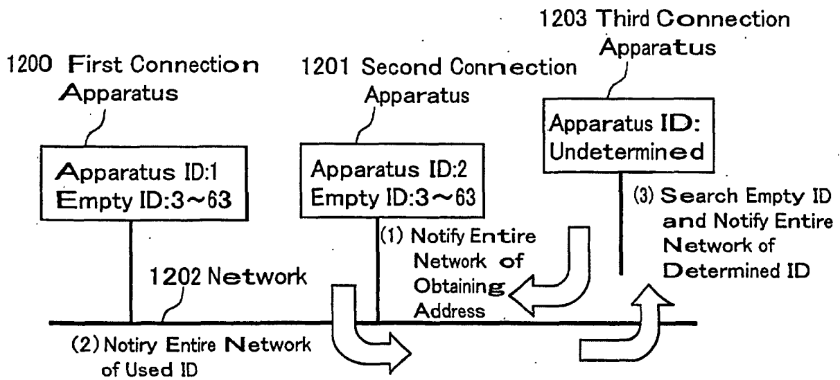
Example of Address Solving Means
