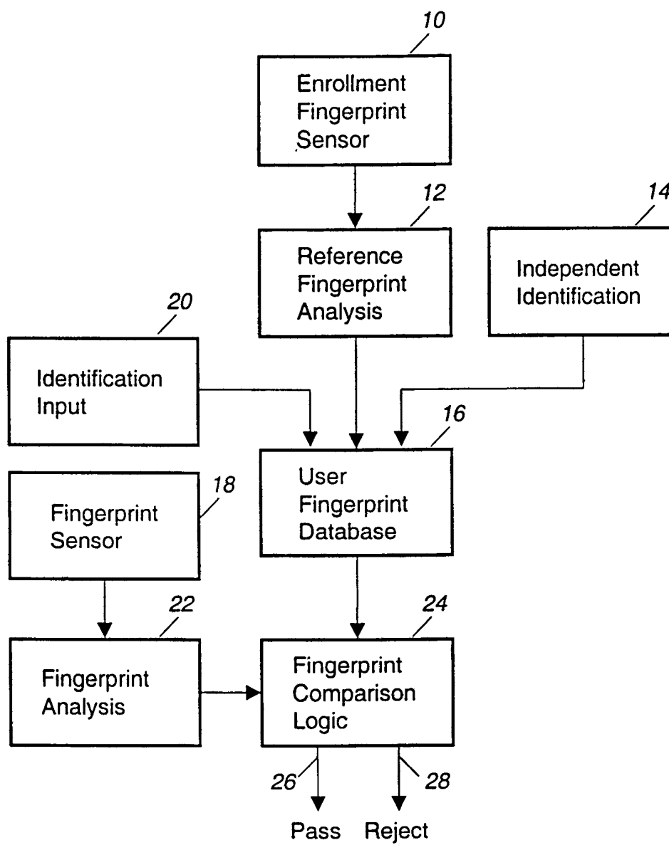
Figure 1 (Prior Art)
