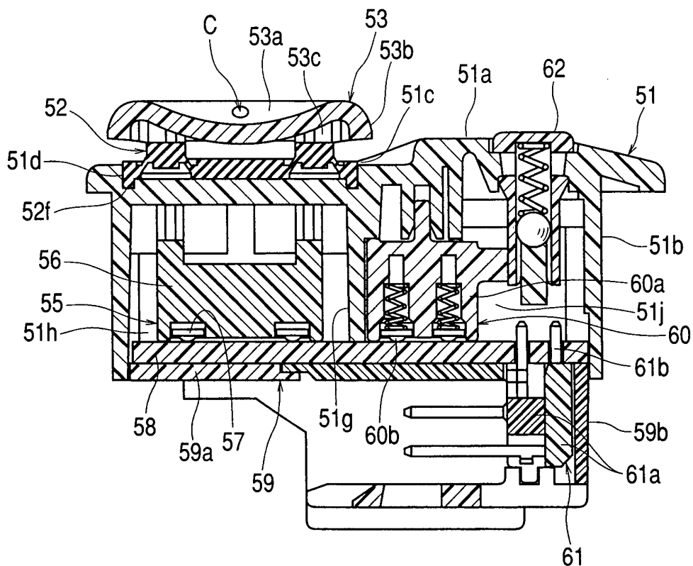
FIG. 8 PRIOR ART
