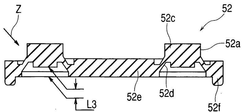
FIG. 9 PRIOR ART
