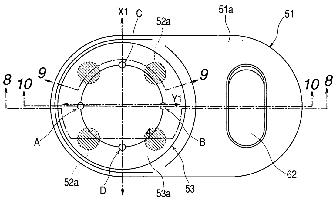
FIG. 7 PRIOR ART
