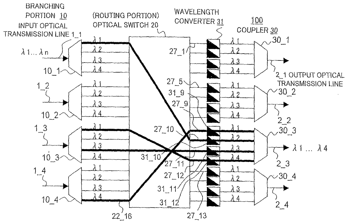
FIG.10A BEFORE FAULT
