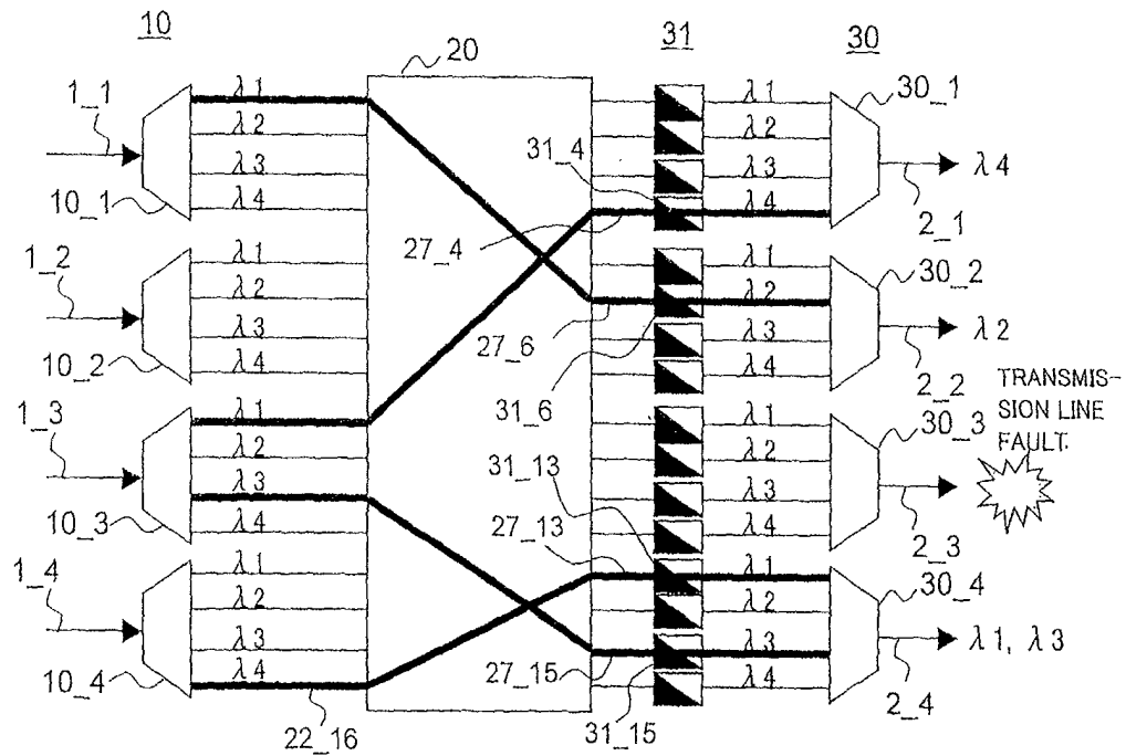
FIG.10B AFTER FAULT
