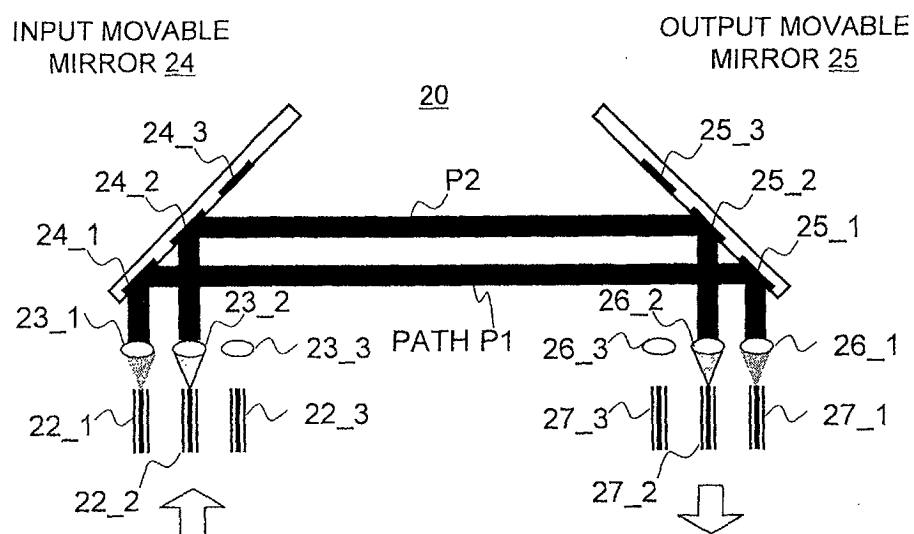
FIG.19B DURING SWITCHOVER
