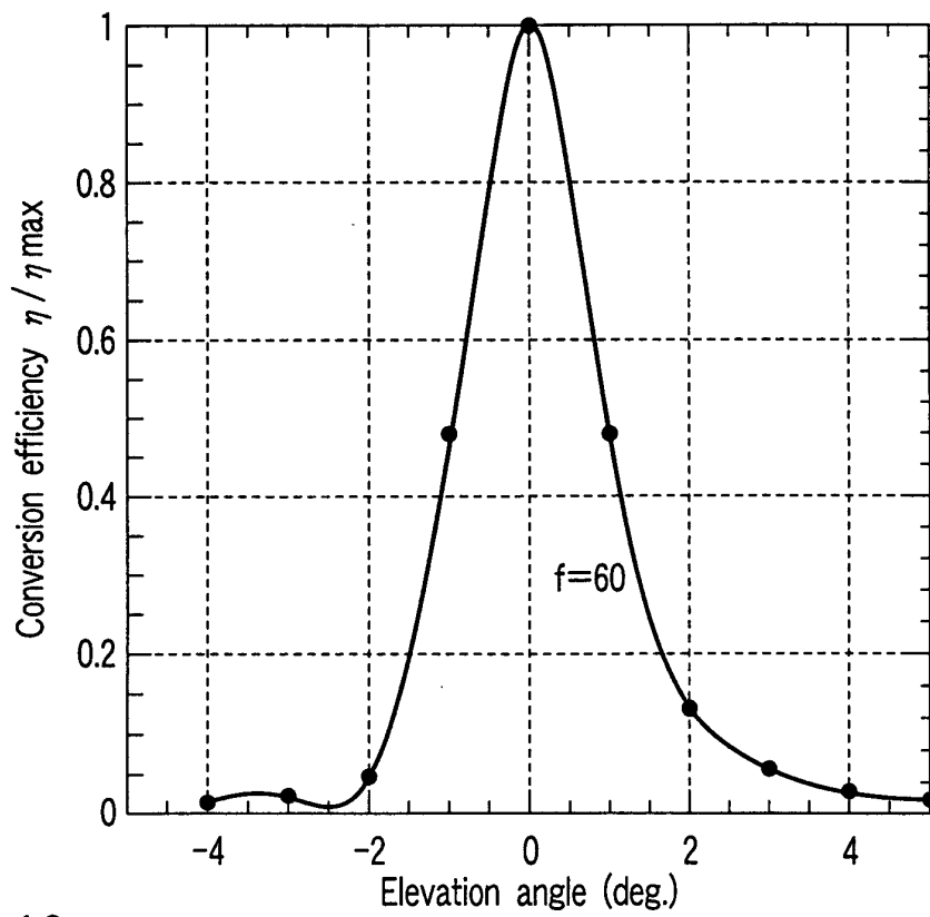
FIG. 12 Rotation angle dependency of SHG conversion efficiency
