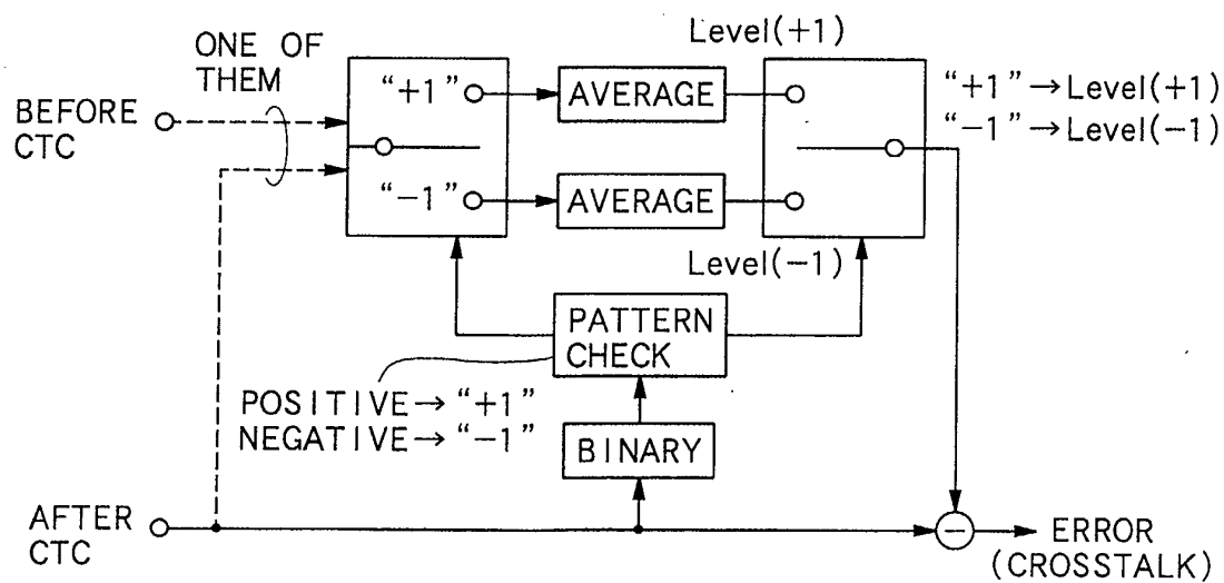
ERROR DETECTION BLOCK DIAGRAM
