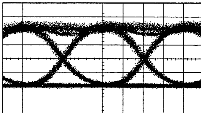
OPTICAL WAVEFORM JUST AFTER TRANSMISSION
