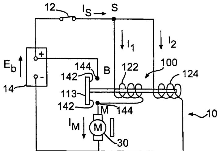
FIG. 3 PRIOR ART
