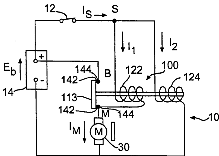
FIG. 4 PRIOR ART
